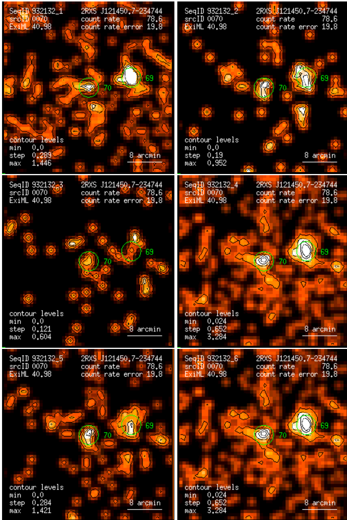
Figure 70: RASS 932132: detection 0070: band rate images, Gaussian filter: (1) PSPC channels 11 – 41, (2) 52 – 90, (3) 91 – 201, (4) 11 – 235, (5) 52 – 201, (6) 11 – 201. Broad band rates in counts/ks. Band rate contour levels in counts/ks/arcmin 2 .
