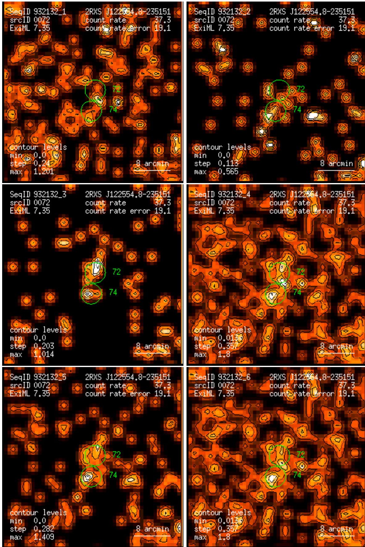
Figure 72: RASS 932132: detection 0072: band rate images, Gaussian filter: (1) PSPC channels 11 – 41, (2) 52 – 90, (3) 91 – 201, (4) 11 – 235, (5) 52 – 201, (6) 11 – 201. Broad band rates in counts/ks. Band rate contour levels in counts/ks/arcmin 2 .
