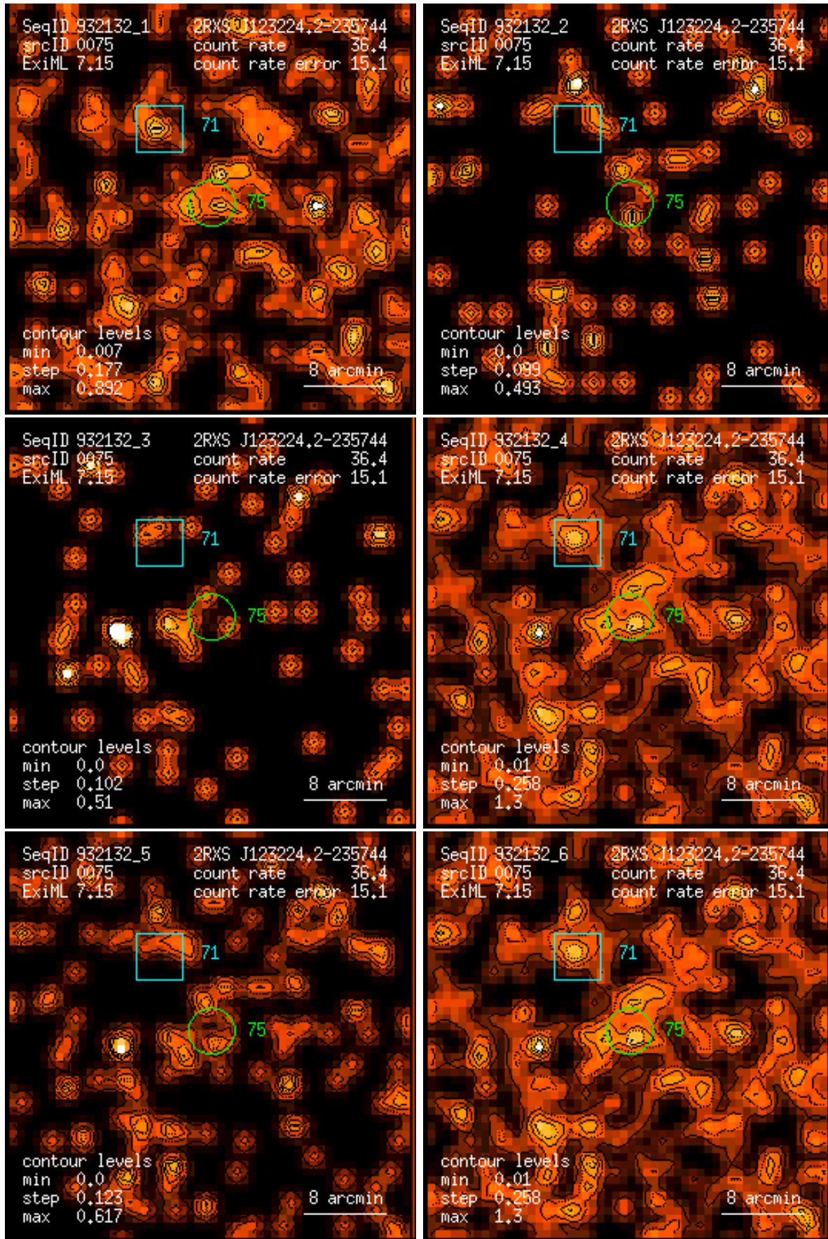
Figure 75: RASS 932132: detection 0075: band rate images, Gaussian filter: (1) PSPC channels 11 – 41, (2) 52 – 90, (3) 91 – 201, (4) 11 – 235, (5) 52 – 201, (6) 11 – 201. Broad band rates in counts/ks. Band rate contour levels in counts/ks/arcmin 2 .
