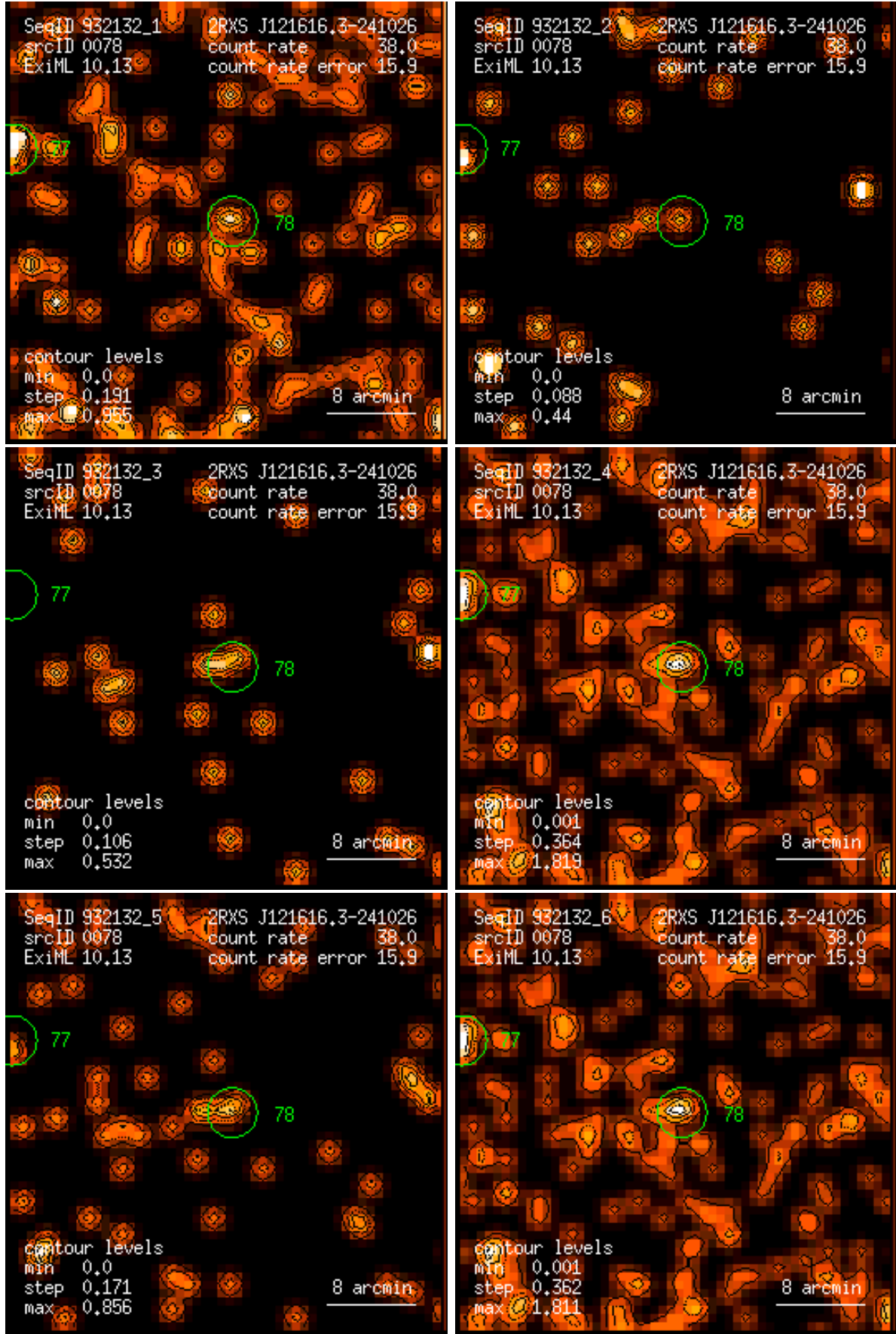
Figure 78: RASS 932132: detection 0078: band rate images, Gaussian filter: (1) PSPC channels 11 – 41, (2) 52 – 90, (3) 91 – 201, (4) 11 – 235, (5) 52 – 201, (6) 11 – 201. Broad band rates in counts/ks. Band rate contour levels in counts/ks/arcmin 2 .
