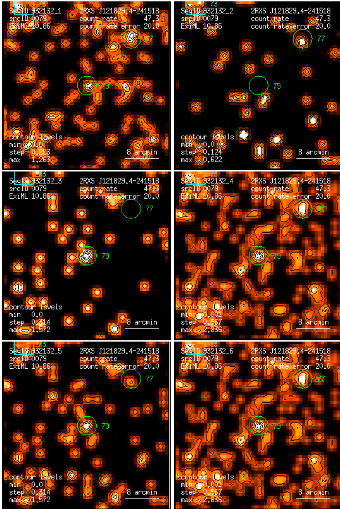
Figure 79: RASS 932132: detection 0079: band rate images, Gaussian filter: (1) PSPC channels 11 – 41, (2) 52 – 90, (3) 91 – 201, (4) 11 – 235, (5) 52 – 201, (6) 11 – 201. Broad band rates in counts/ks. Band rate contour levels in counts/ks/arcmin 2 .
