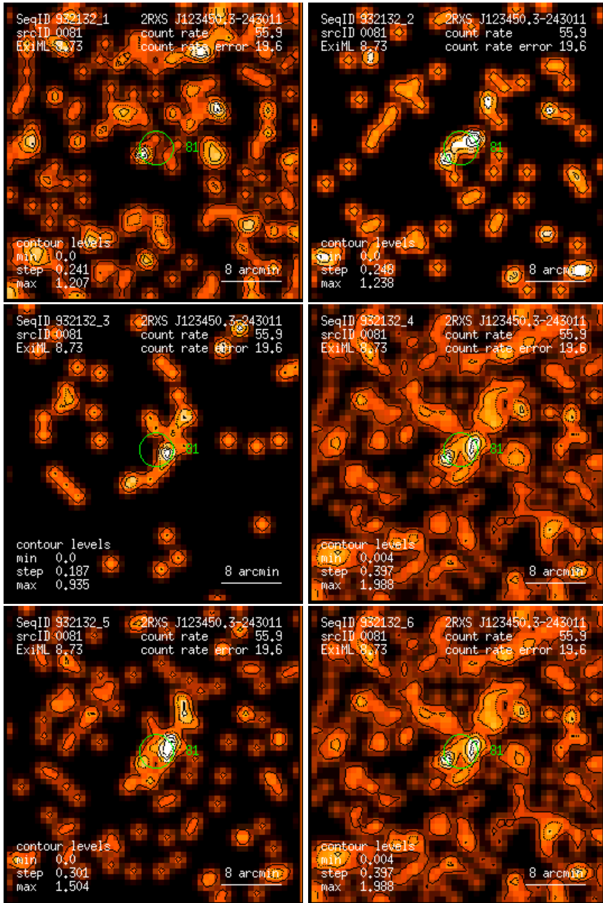
Figure 81: RASS 932132: detection 0081: band rate images, Gaussian filter: (1) PSPC channels 11 – 41, (2) 52 – 90, (3) 91 – 201, (4) 11 – 235, (5) 52 – 201, (6) 11 – 201. Broad band rates in counts/ks. Band rate contour levels in counts/ks/arcmin 2 .
