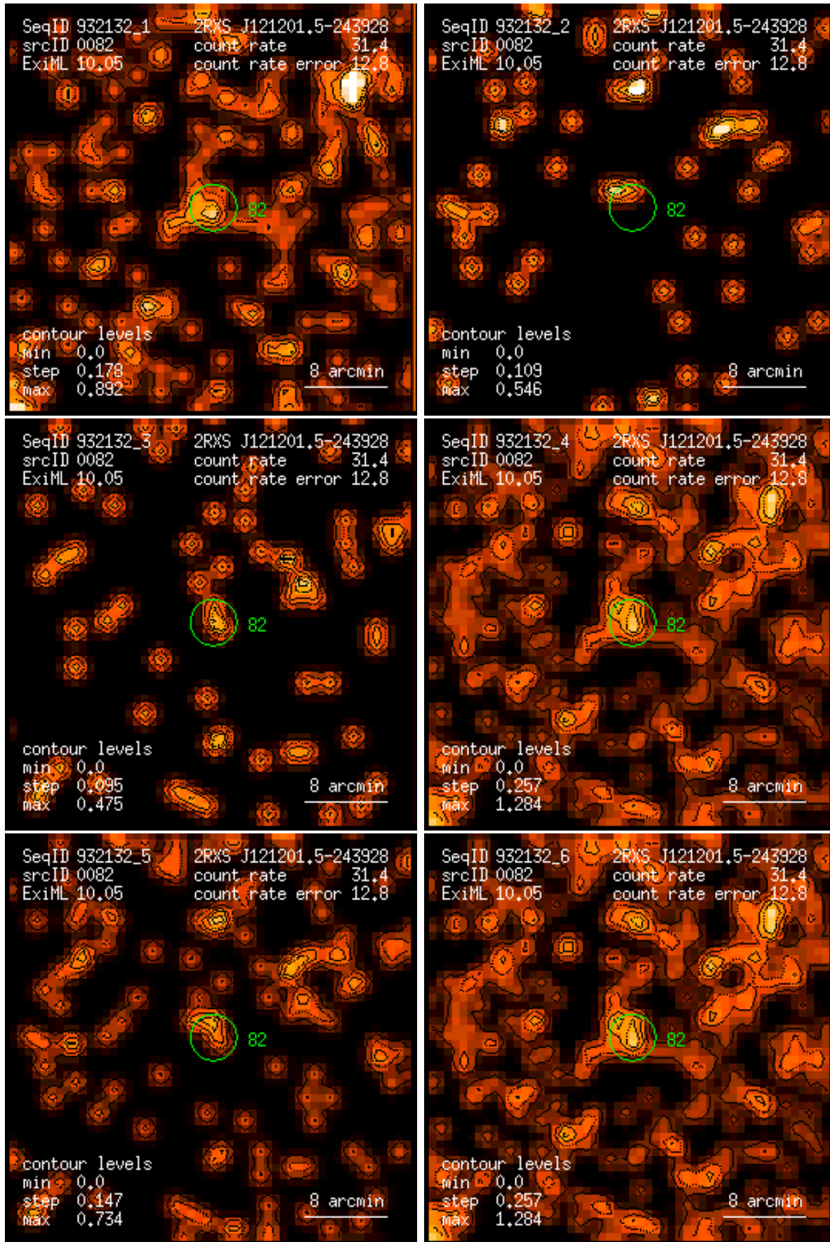
Figure 82: RASS 932132: detection 0082: band rate images, Gaussian filter: (1) PSPC channels 11 – 41, (2) 52 – 90, (3) 91 – 201, (4) 11 – 235, (5) 52 – 201, (6) 11 – 201. Broad band rates in counts/ks. Band rate contour levels in counts/ks/arcmin 2 .
