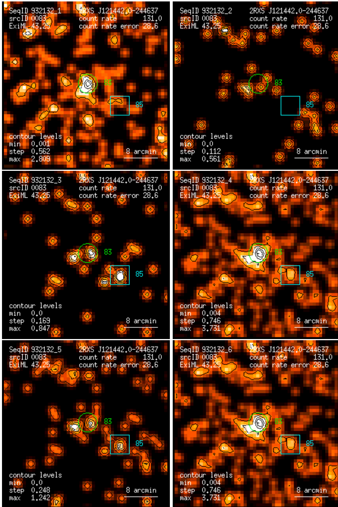
Figure 83: RASS 932132: detection 0083: band rate images, Gaussian filter: (1) PSPC channels 11 – 41, (2) 52 – 90, (3) 91 – 201, (4) 11 – 235, (5) 52 – 201, (6) 11 – 201. Broad band rates in counts/ks. Band rate contour levels in counts/ks/arcmin 2 .
