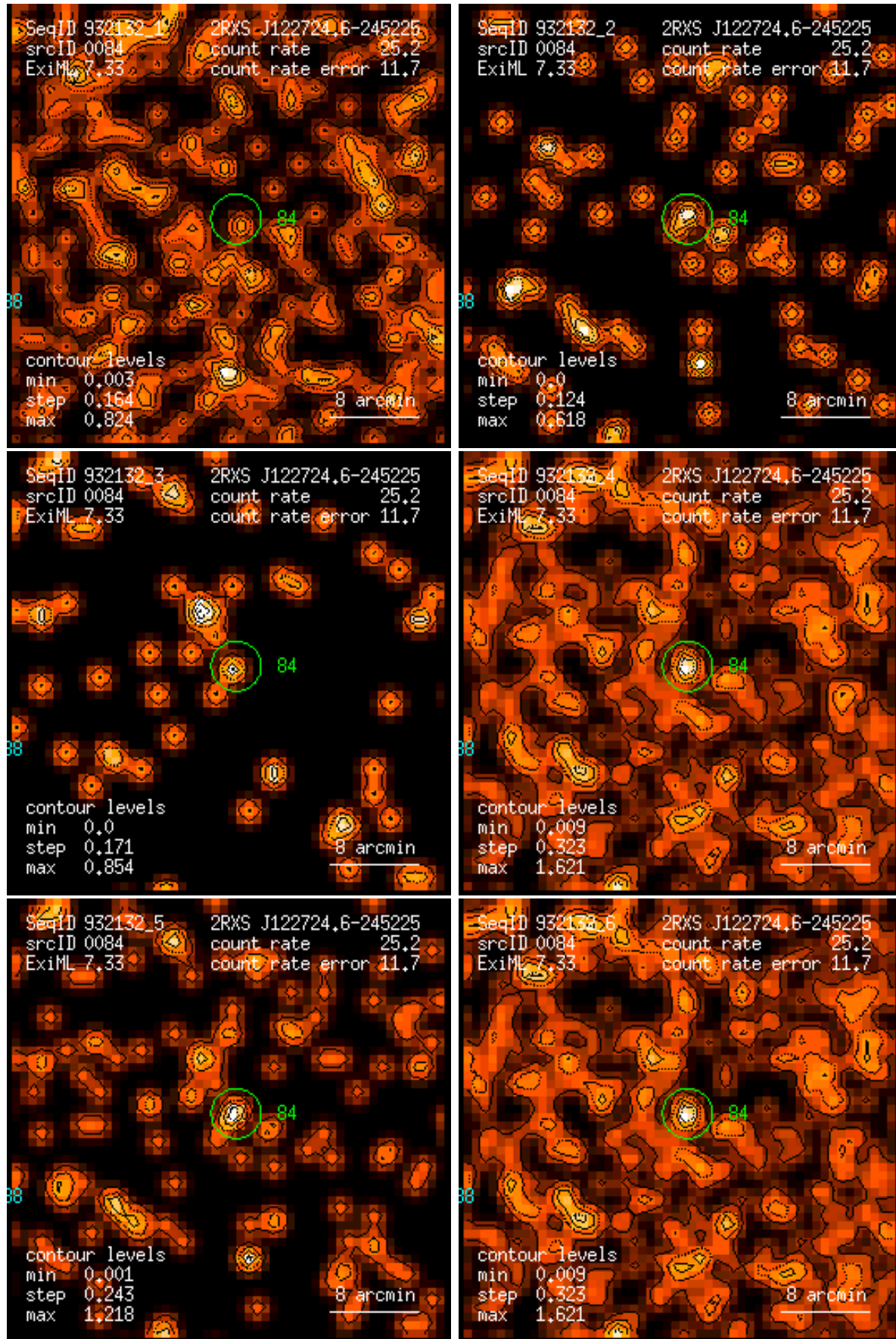
Figure 84: RASS 932132: detection 0084: band rate images, Gaussian filter: (1) PSPC channels 11 – 41, (2) 52 – 90, (3) 91 – 201, (4) 11 – 235, (5) 52 – 201, (6) 11 – 201. Broad band rates in counts/ks. Band rate contour levels in counts/ks/arcmin 2 .
