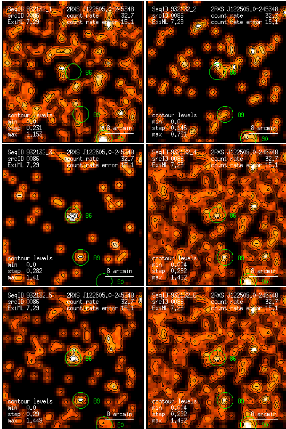
Figure 86: RASS 932132: detection 0086: band rate images, Gaussian filter: (1) PSPC channels 11 – 41, (2) 52 – 90, (3) 91 – 201, (4) 11 – 235, (5) 52 – 201, (6) 11 – 201. Broad band rates in counts/ks. Band rate contour levels in counts/ks/arcmin 2 .
