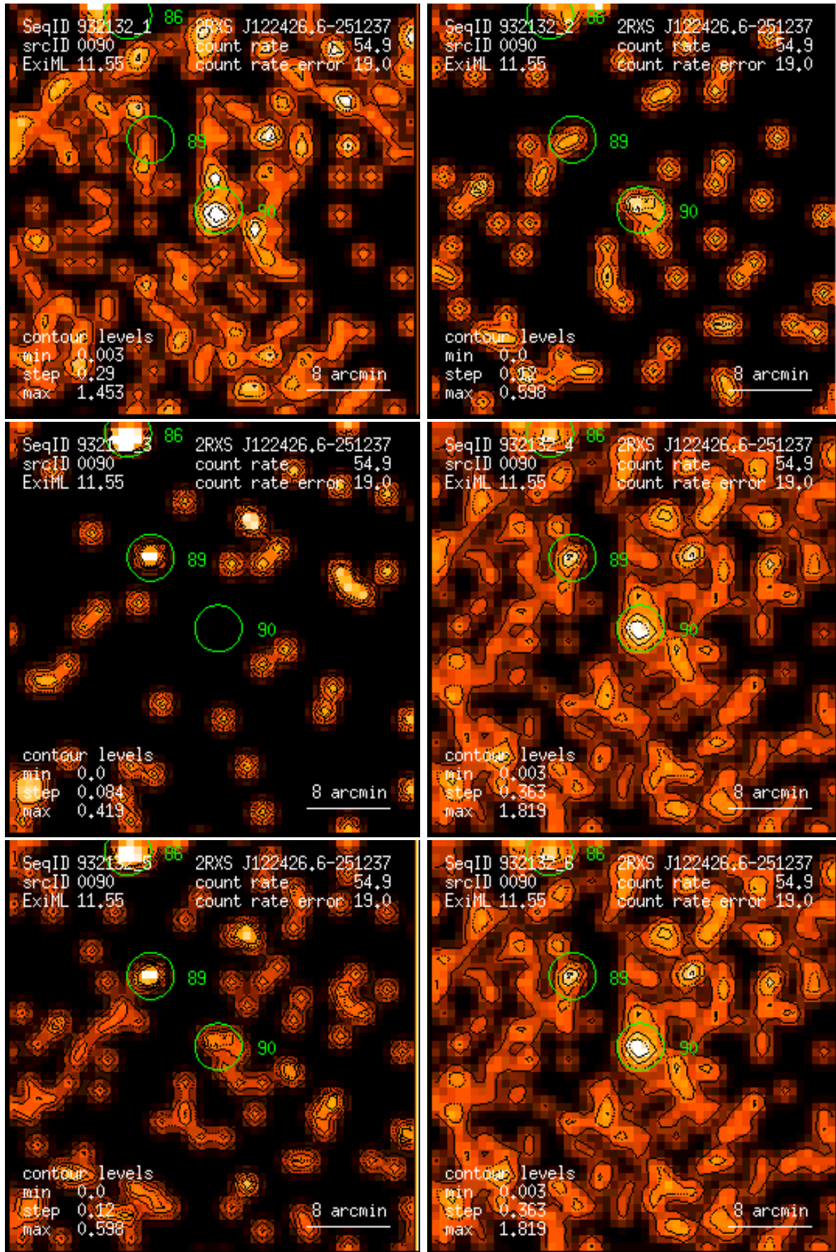
Figure 90: RASS 932132: detection 0090: band rate images, Gaussian filter: (1) PSPC channels 11 – 41, (2) 52 – 90, (3) 91 – 201, (4) 11 – 235, (5) 52 – 201, (6) 11 – 201. Broad band rates in counts/ks. Band rate contour levels in counts/ks/arcmin 2 .
