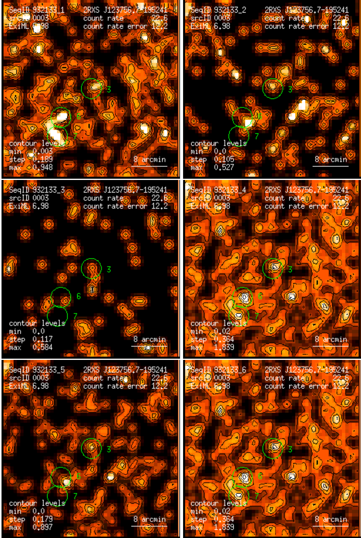
Figure 3: RASS 932133: detection 0003: band rate images, Gaussian filter: (1) PSPC channels 11 – 41, (2) 52 – 90, (3) 91 – 201, (4) 11 – 235, (5) 52 – 201, (6) 11 – 201. Broad band rates in counts/ks. Band rate contour levels in counts/ks/arcmin 2 .
