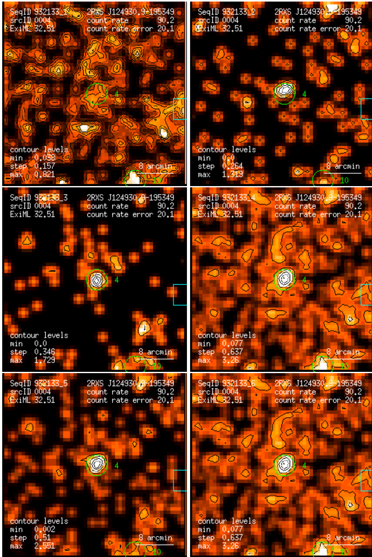
Figure 4: RASS 932133: detection 0004: band rate images, Gaussian filter: (1) PSPC channels 11 – 41, (2) 52 – 90, (3) 91 – 201, (4) 11 – 235, (5) 52 – 201, (6) 11 – 201. Broad band rates in counts/ks. Band rate contour levels in counts/ks/arcmin 2 .
