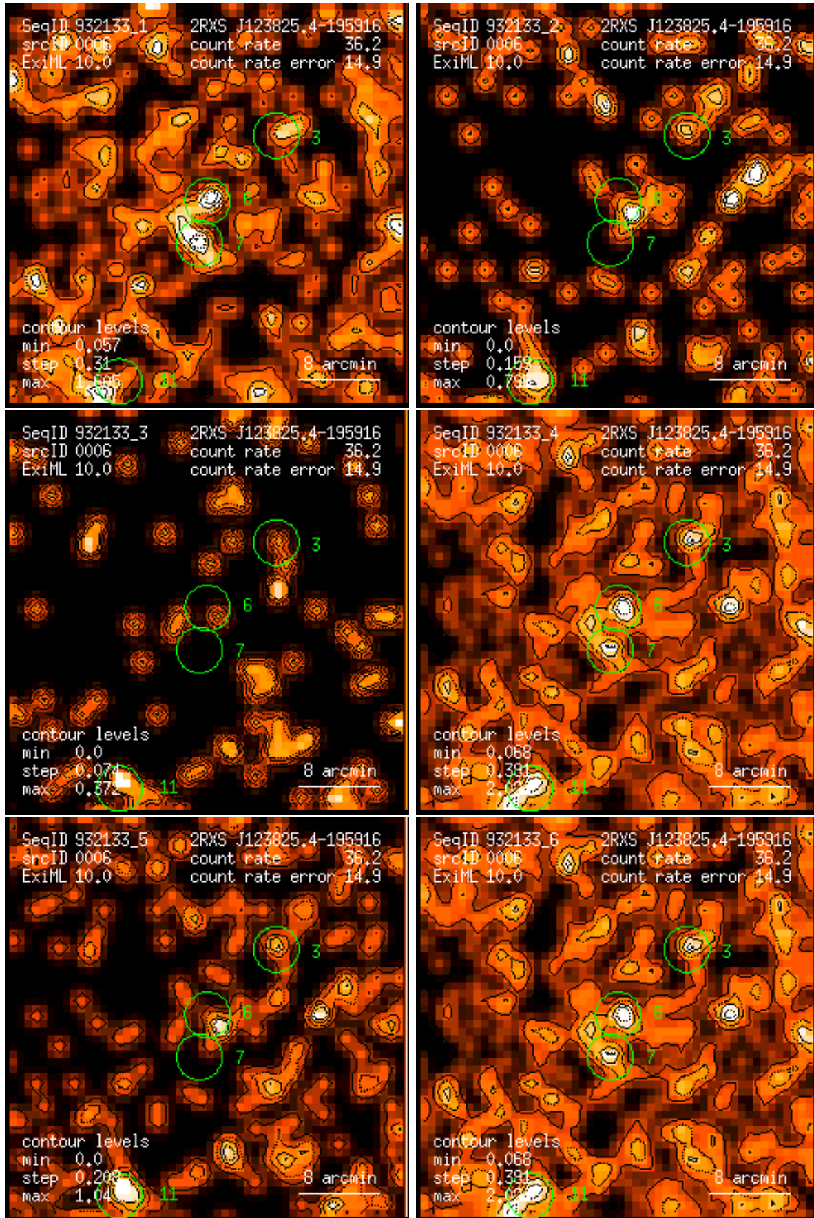
Figure 6: RASS 932133: detection 0006: band rate images, Gaussian filter: (1) PSPC channels 11 – 41, (2) 52 – 90, (3) 91 – 201, (4) 11 – 235, (5) 52 – 201, (6) 11 – 201. Broad band rates in counts/ks. Band rate contour levels in counts/ks/arcmin 2 .
