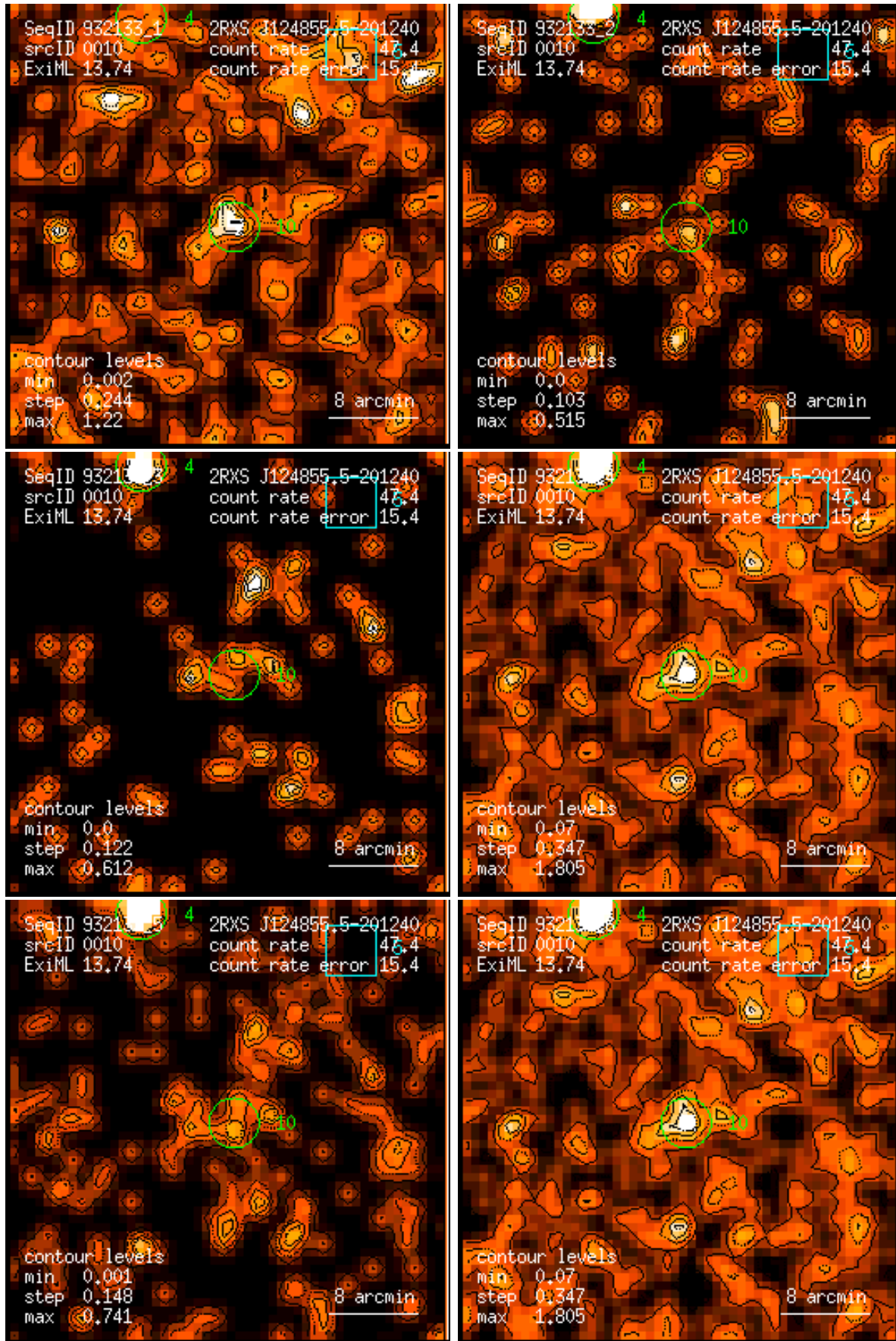
Figure 10: RASS 932133: detection 0010: band rate images, Gaussian filter: (1) PSPC channels 11 – 41, (2) 52 – 90, (3) 91 – 201, (4) 11 – 235, (5) 52 – 201, (6) 11 – 201. Broad band rates in counts/ks. Band rate contour levels in counts/ks/arcmin 2 .
