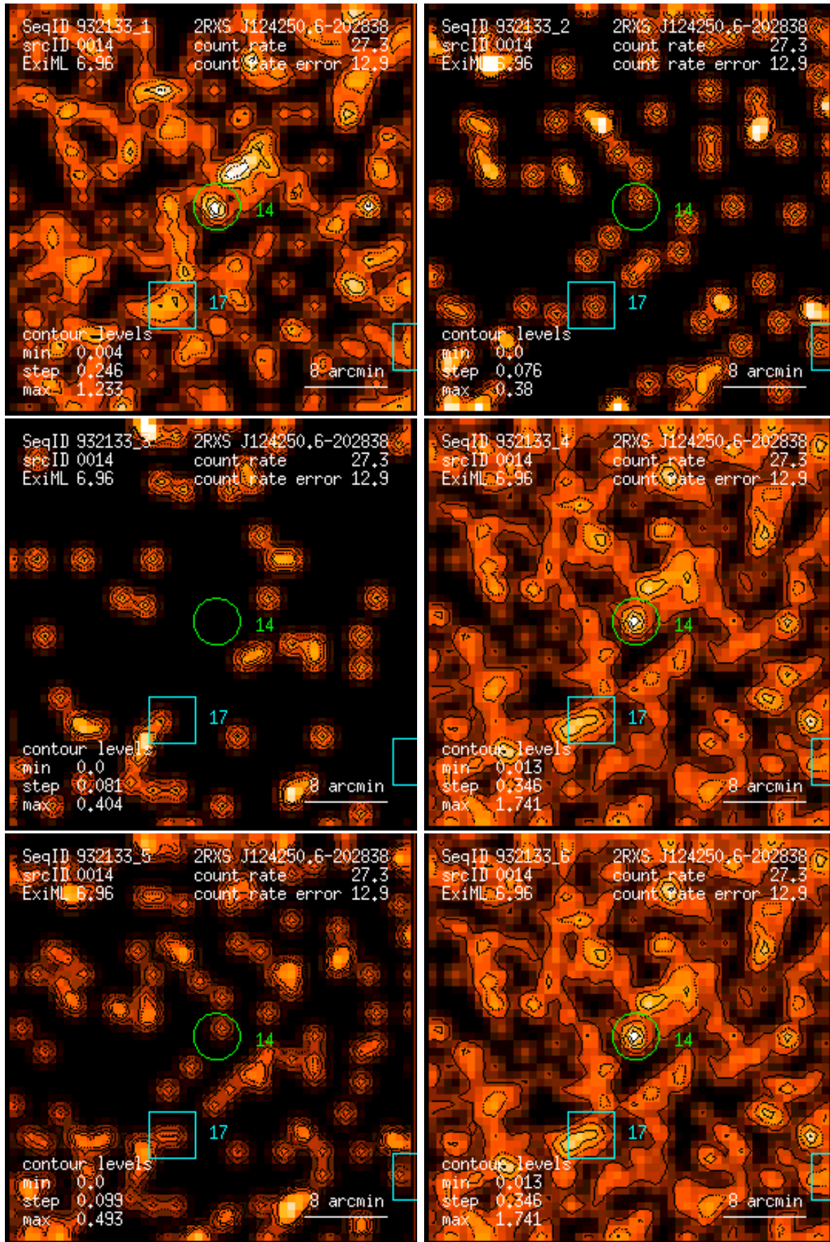
Figure 14: RASS 932133: detection 0014: band rate images, Gaussian filter: (1) PSPC channels 11 – 41, (2) 52 – 90, (3) 91 – 201, (4) 11 – 235, (5) 52 – 201, (6) 11 – 201. Broad band rates in counts/ks. Band rate contour levels in counts/ks/arcmin 2 .
