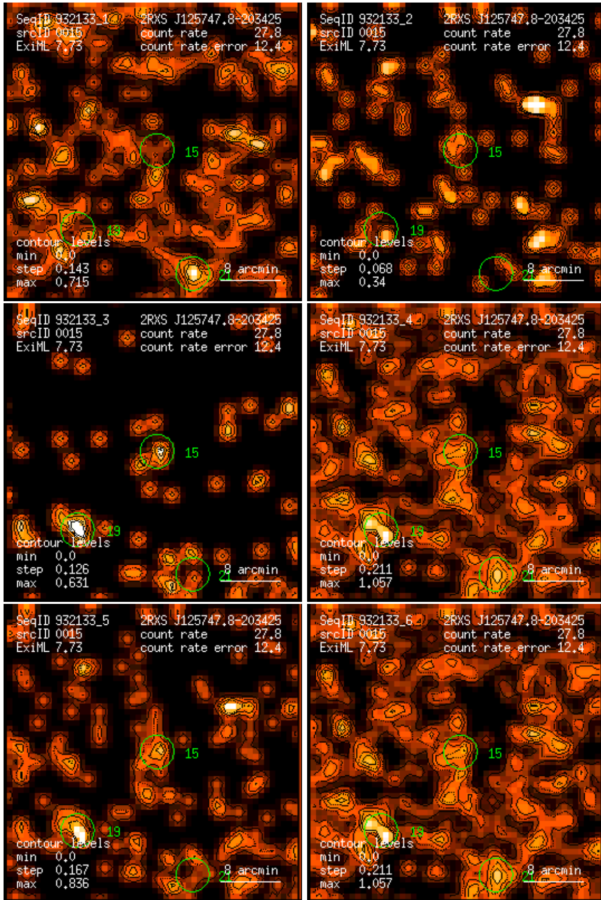
Figure 15: RASS 932133: detection 0015: band rate images, Gaussian filter: (1) PSPC channels 11 – 41, (2) 52 – 90, (3) 91 – 201, (4) 11 – 235, (5) 52 – 201, (6) 11 – 201. Broad band rates in counts/ks. Band rate contour levels in counts/ks/arcmin 2 .
