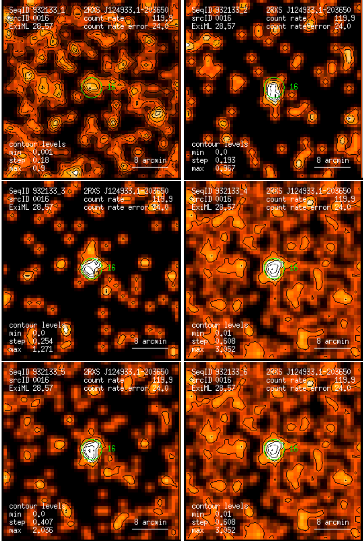
Figure 16: RASS 932133: detection 0016: band rate images, Gaussian filter: (1) PSPC channels 11 – 41, (2) 52 – 90, (3) 91 – 201, (4) 11 – 235, (5) 52 – 201, (6) 11 – 201. Broad band rates in counts/ks. Band rate contour levels in counts/ks/arcmin 2 .
