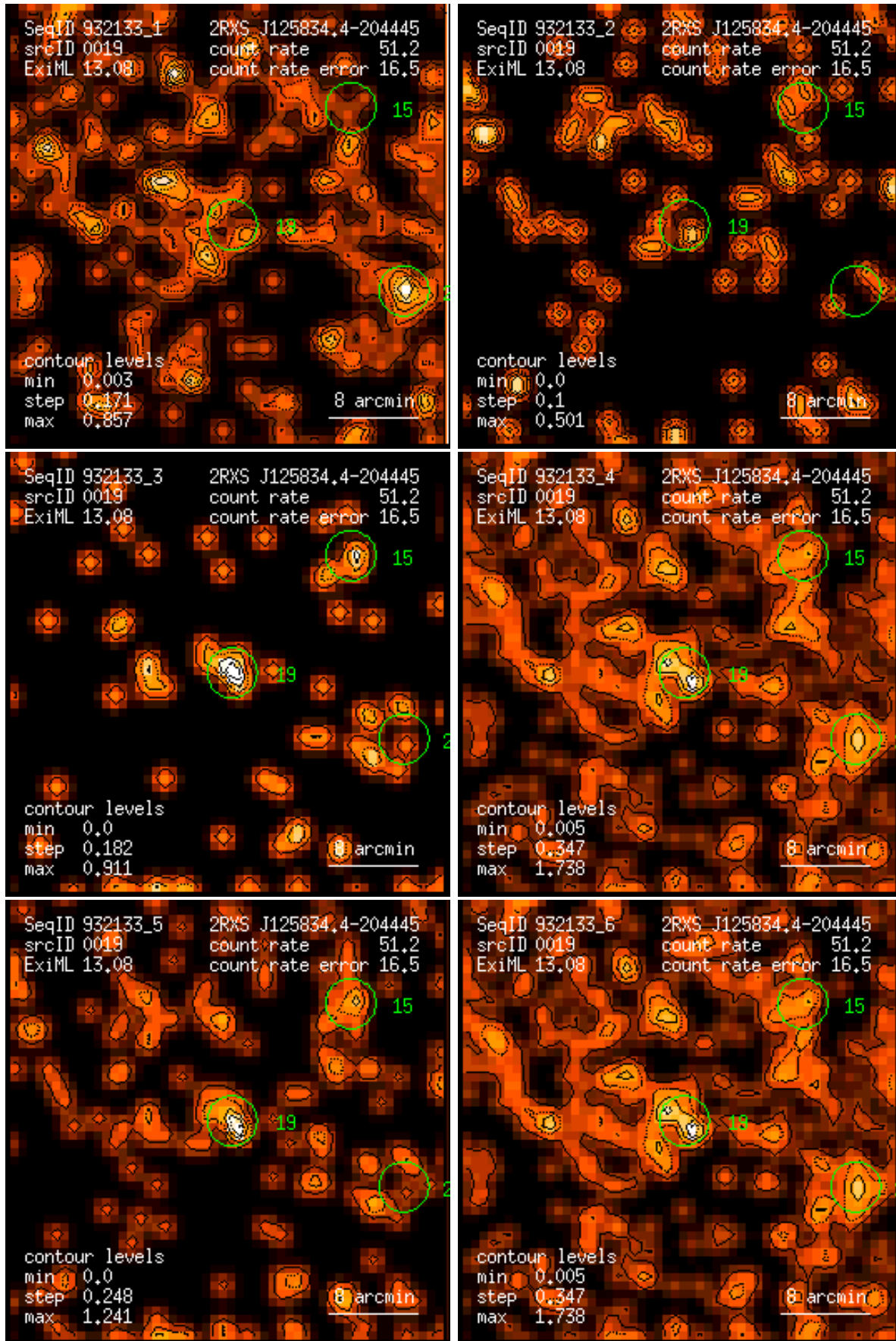
Figure 19: RASS 932133: detection 0019: band rate images, Gaussian filter: (1) PSPC channels 11 – 41, (2) 52 – 90, (3) 91 – 201, (4) 11 – 235, (5) 52 – 201, (6) 11 – 201. Broad band rates in counts/ks. Band rate contour levels in counts/ks/arcmin 2 .
