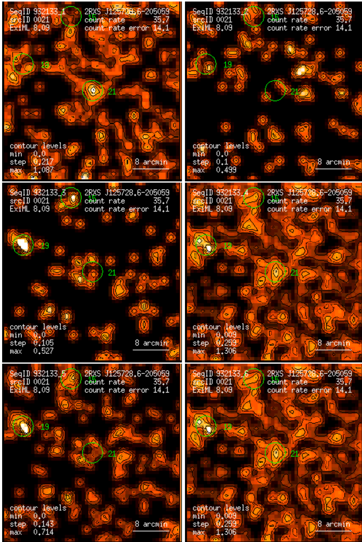
Figure 21: RASS 932133: detection 0021: band rate images, Gaussian filter: (1) PSPC channels 11 – 41, (2) 52 – 90, (3) 91 – 201, (4) 11 – 235, (5) 52 – 201, (6) 11 – 201. Broad band rates in counts/ks. Band rate contour levels in counts/ks/arcmin 2 .
