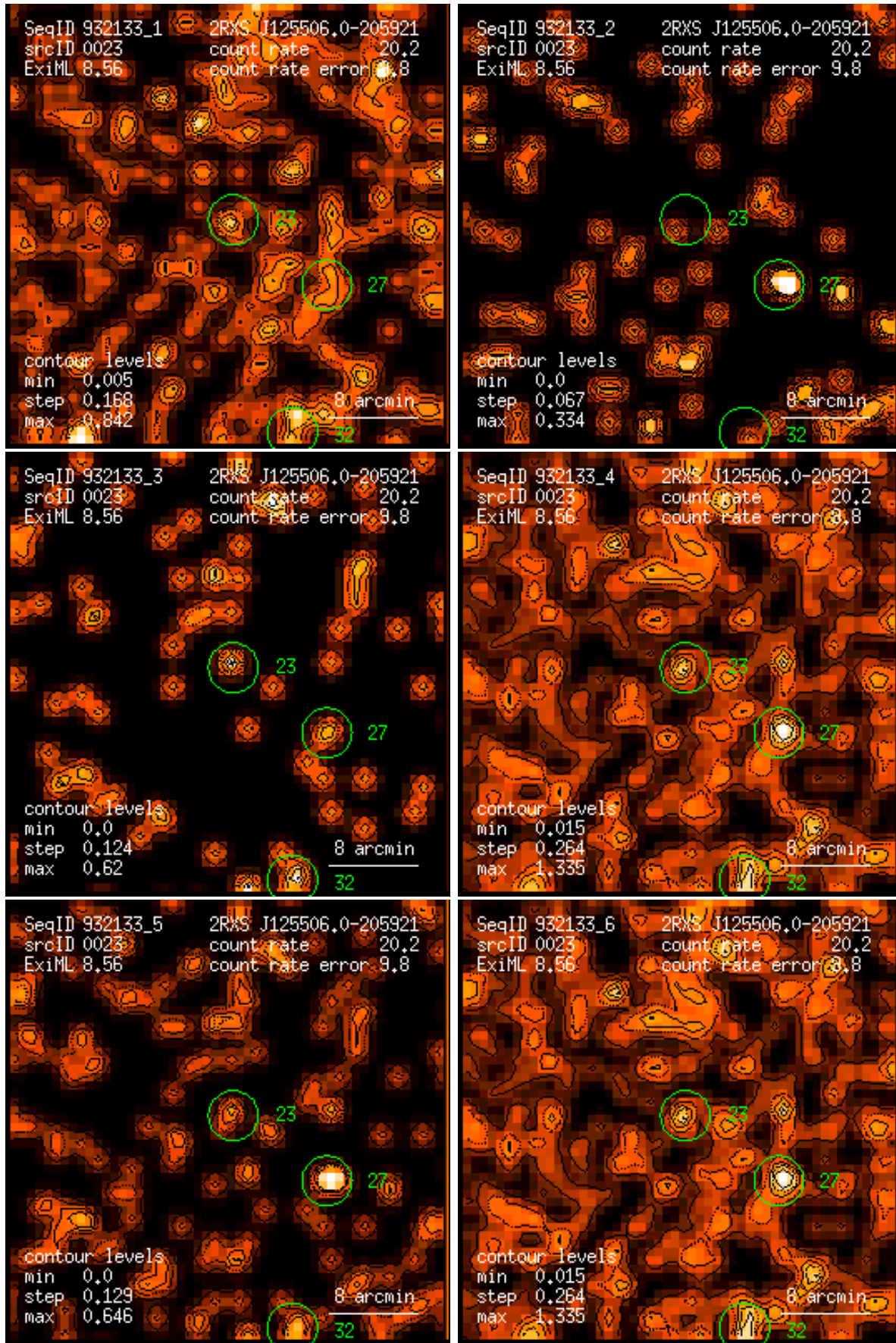
Figure 23: RASS 932133: detection 0023: band rate images, Gaussian filter: (1) PSPC channels 11 – 41, (2) 52 – 90, (3) 91 – 201, (4) 11 – 235, (5) 52 – 201, (6) 11 – 201. Broad band rates in counts/ks. Band rate contour levels in counts/ks/arcmin 2 .
