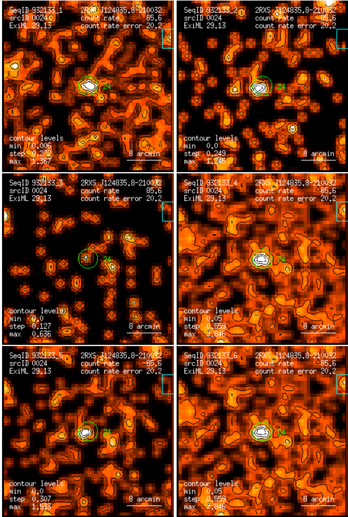
Figure 24: RASS 932133: detection 0024: band rate images, Gaussian filter: (1) PSPC channels 11 – 41, (2) 52 – 90, (3) 91 – 201, (4) 11 – 235, (5) 52 – 201, (6) 11 – 201. Broad band rates in counts/ks. Band rate contour levels in counts/ks/arcmin 2 .
