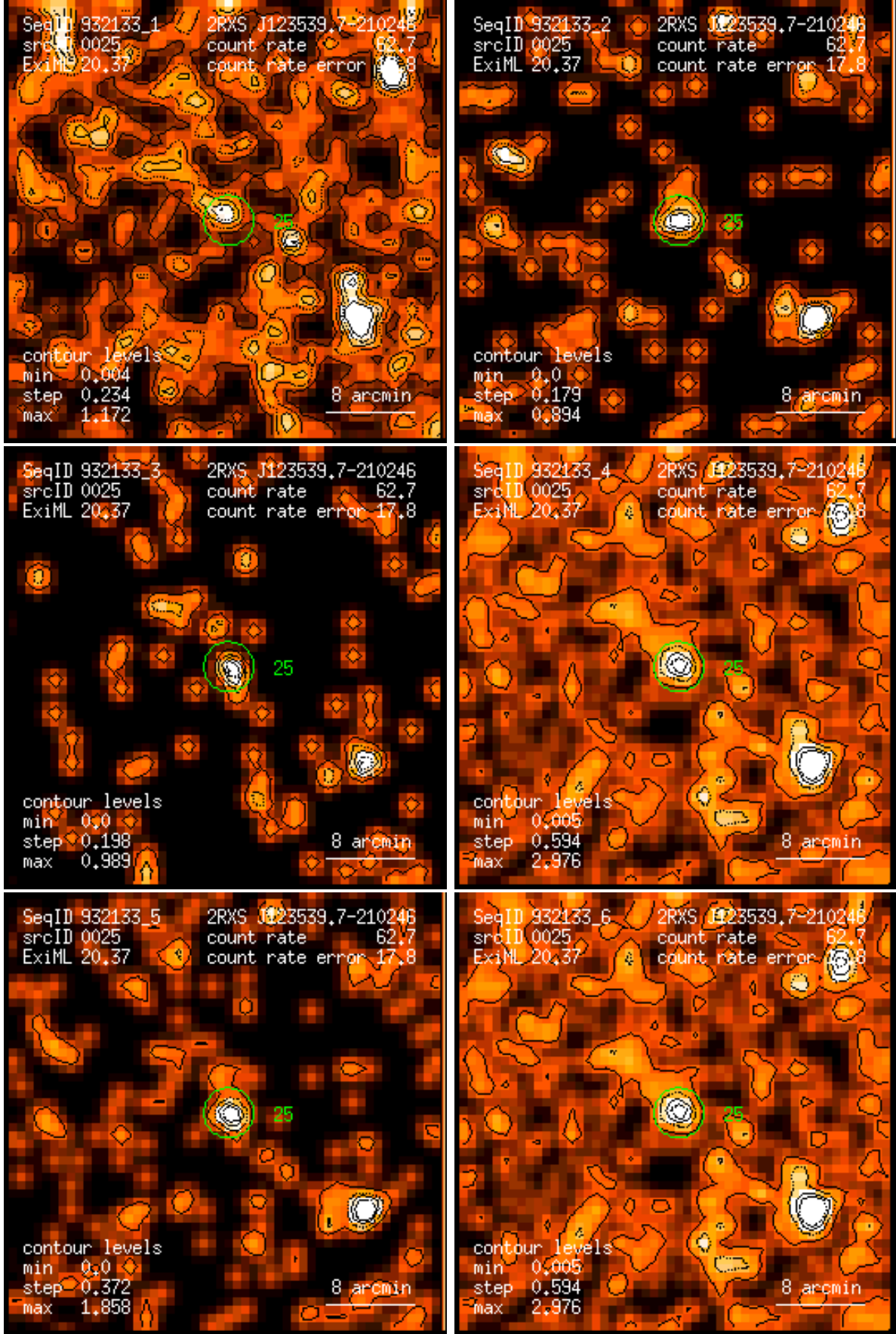
Figure 25: RASS 932133: detection 0025: band rate images, Gaussian filter: (1) PSPC channels 11 – 41, (2) 52 – 90, (3) 91 – 201, (4) 11 – 235, (5) 52 – 201, (6) 11 – 201. Broad band rates in counts/ks. Band rate contour levels in counts/ks/arcmin 2 .
