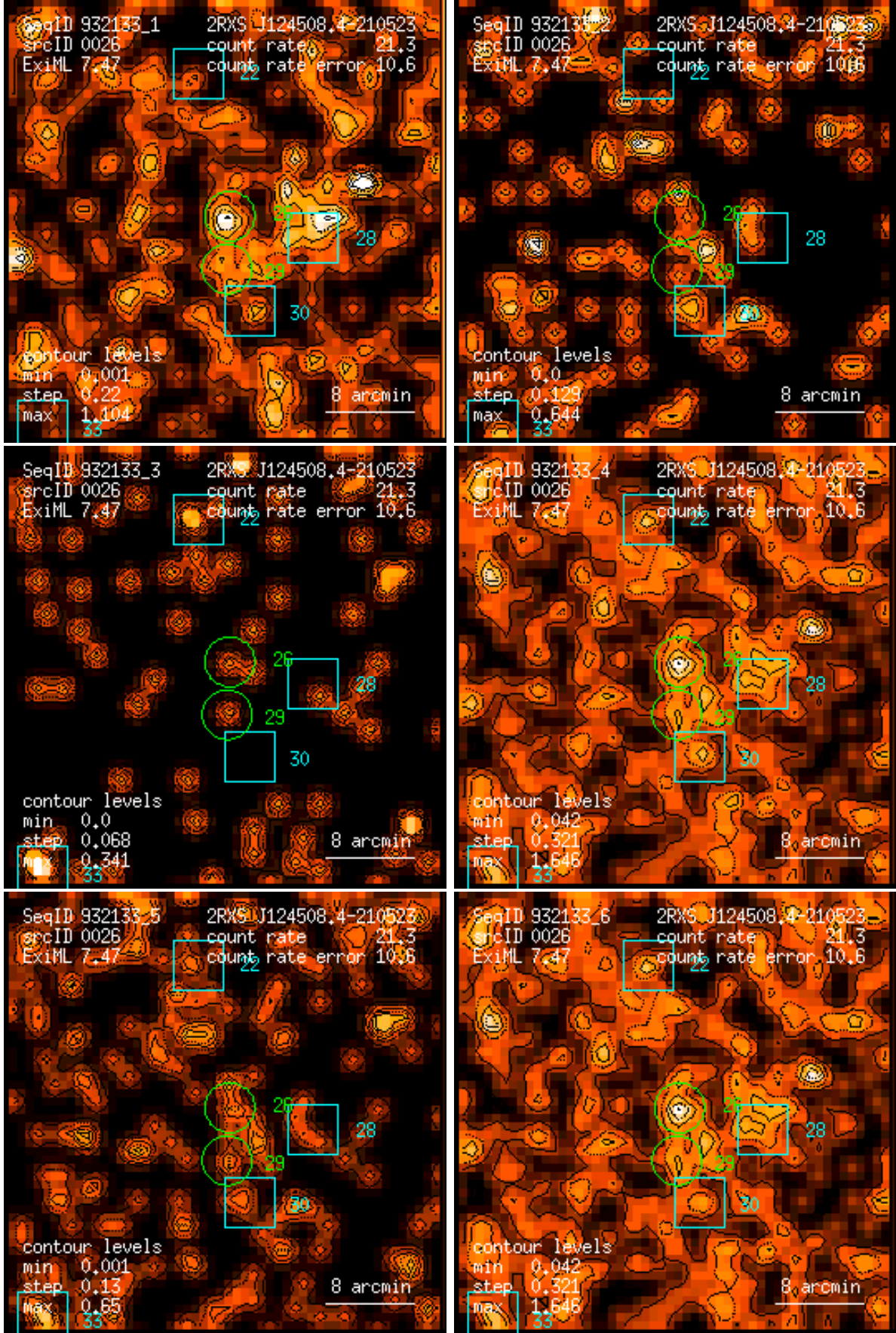
Figure 26: RASS 932133: detection 0026: band rate images, Gaussian filter: (1) PSPC channels 11 – 41, (2) 52 – 90, (3) 91 – 201, (4) 11 – 235, (5) 52 – 201, (6) 11 – 201. Broad band rates in counts/ks. Band rate contour levels in counts/ks/arcmin 2 .
