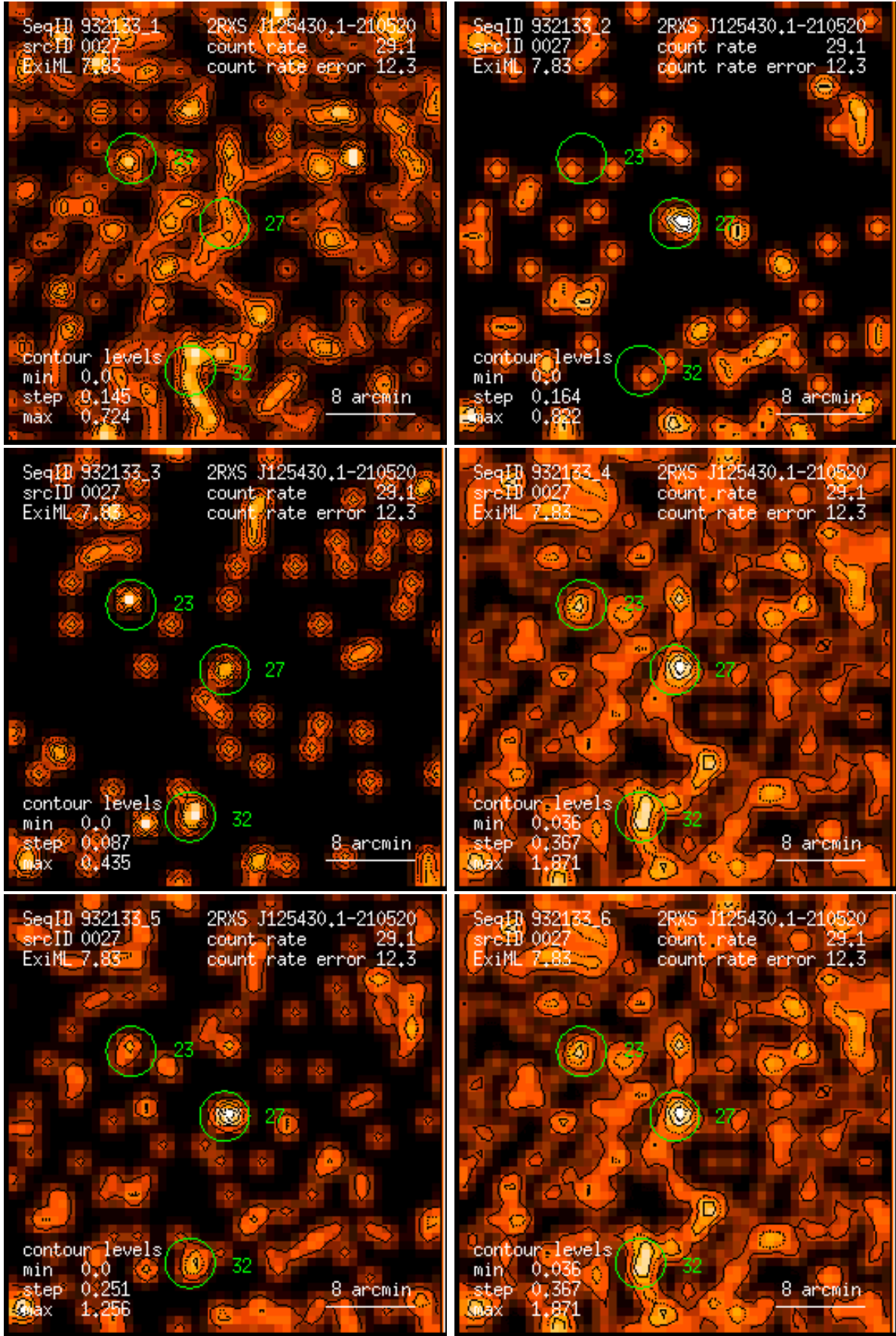
Figure 27: RASS 932133: detection 0027: band rate images, Gaussian filter: (1) PSPC channels 11 – 41, (2) 52 – 90, (3) 91 – 201, (4) 11 – 235, (5) 52 – 201, (6) 11 – 201. Broad band rates in counts/ks. Band rate contour levels in counts/ks/arcmin 2 .
