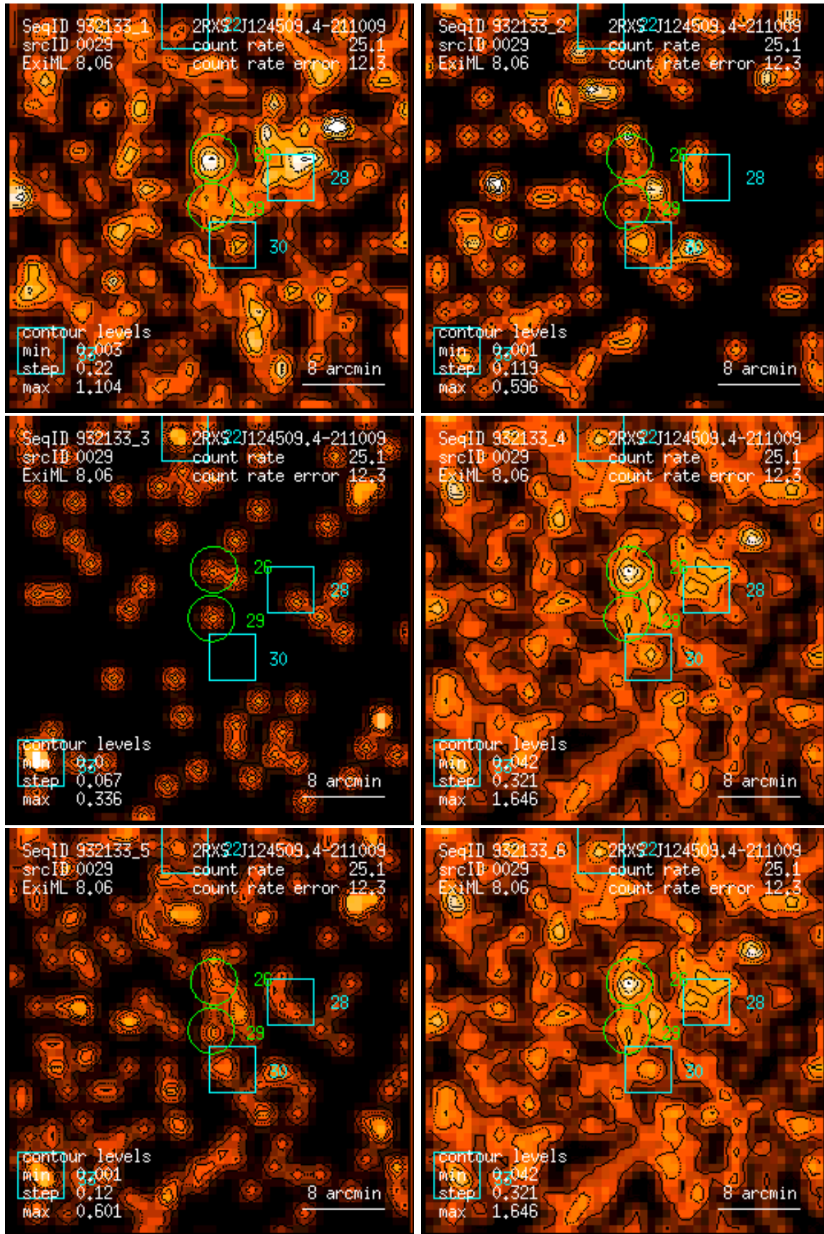
Figure 29: RASS 932133: detection 0029: band rate images, Gaussian filter: (1) PSPC channels 11 – 41, (2) 52 – 90, (3) 91 – 201, (4) 11 – 235, (5) 52 – 201, (6) 11 – 201. Broad band rates in counts/ks. Band rate contour levels in counts/ks/arcmin 2 .
