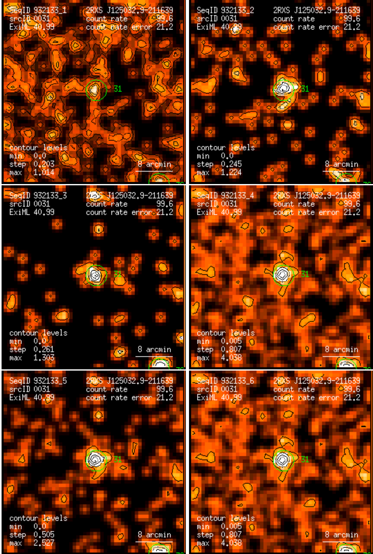
Figure 31: RASS 932133: detection 0031: band rate images, Gaussian filter: (1) PSPC channels 11 – 41, (2) 52 – 90, (3) 91 – 201, (4) 11 – 235, (5) 52 – 201, (6) 11 – 201. Broad band rates in counts/ks. Band rate contour levels in counts/ks/arcmin 2 .
