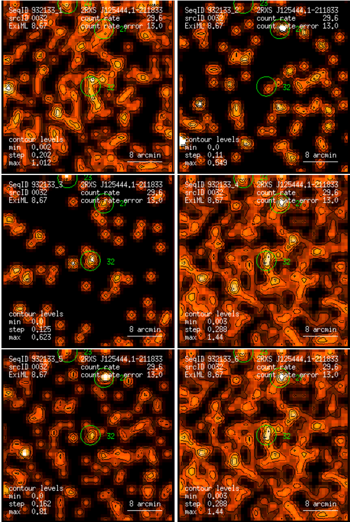
Figure 32: RASS 932133: detection 0032: band rate images, Gaussian filter: (1) PSPC channels 11 – 41, (2) 52 – 90, (3) 91 – 201, (4) 11 – 235, (5) 52 – 201, (6) 11 – 201. Broad band rates in counts/ks. Band rate contour levels in counts/ks/arcmin 2 .
