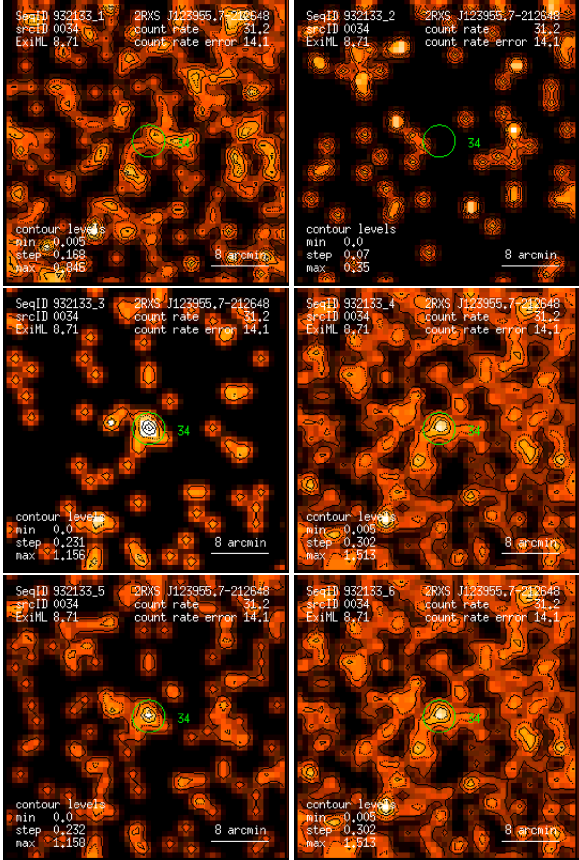
Figure 34: RASS 932133: detection 0034: band rate images, Gaussian filter: (1) PSPC channels 11 – 41, (2) 52 – 90, (3) 91 – 201, (4) 11 – 235, (5) 52 – 201, (6) 11 – 201. Broad band rates in counts/ks. Band rate contour levels in counts/ks/arcmin 2 .
