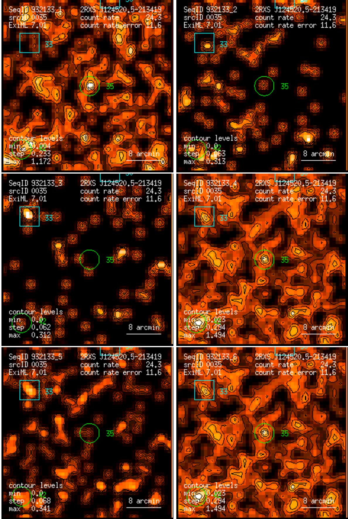
Figure 35: RASS 932133: detection 0035: band rate images, Gaussian filter: (1) PSPC channels 11 – 41, (2) 52 – 90, (3) 91 – 201, (4) 11 – 235, (5) 52 – 201, (6) 11 – 201. Broad band rates in counts/ks. Band rate contour levels in counts/ks/arcmin 2 .
