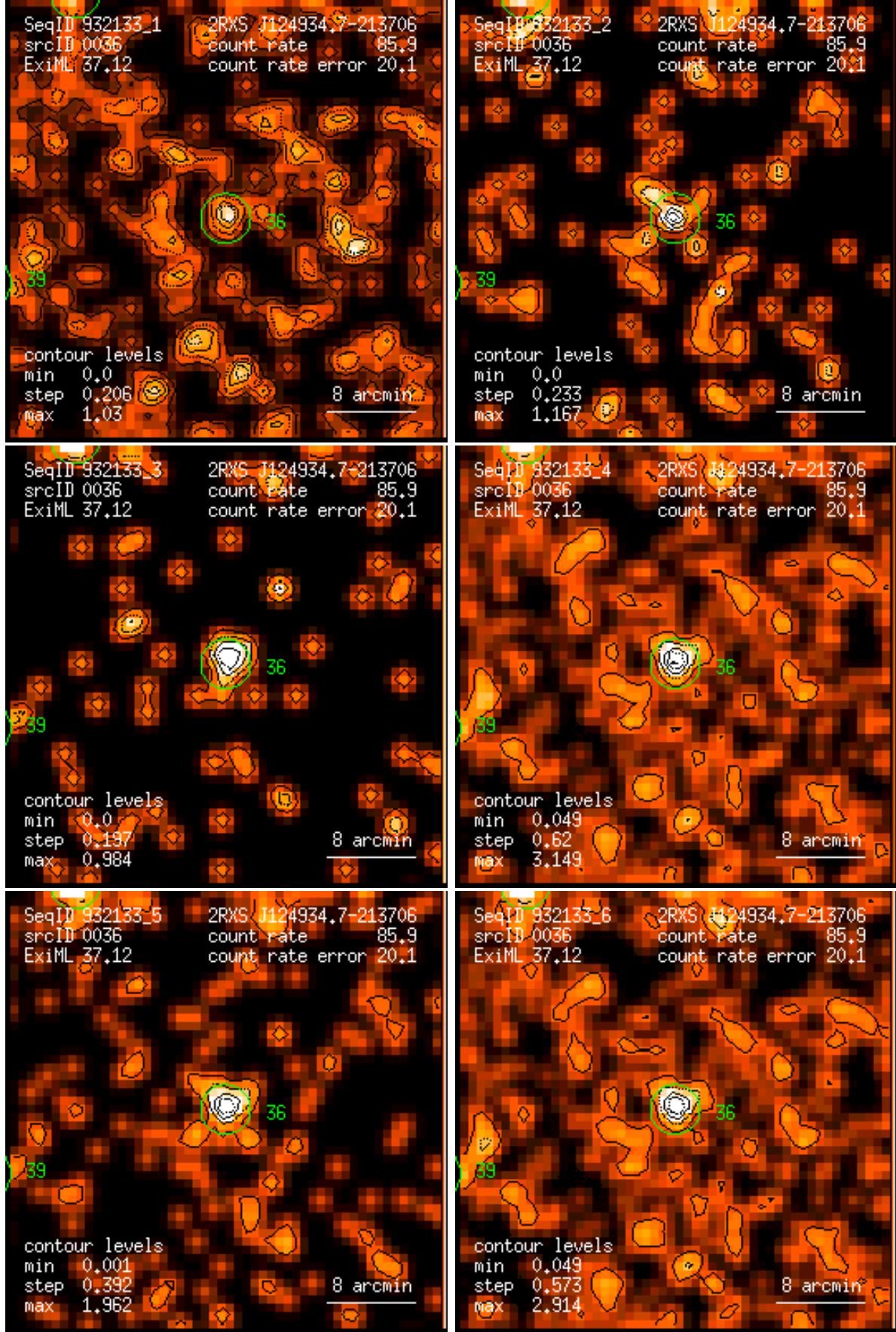
Figure 36: RASS 932133: detection 0036: band rate images, Gaussian filter: (1) PSPC channels 11 – 41, (2) 52 – 90, (3) 91 – 201, (4) 11 – 235, (5) 52 – 201, (6) 11 – 201. Broad band rates in counts/ks. Band rate contour levels in counts/ks/arcmin 2 .
