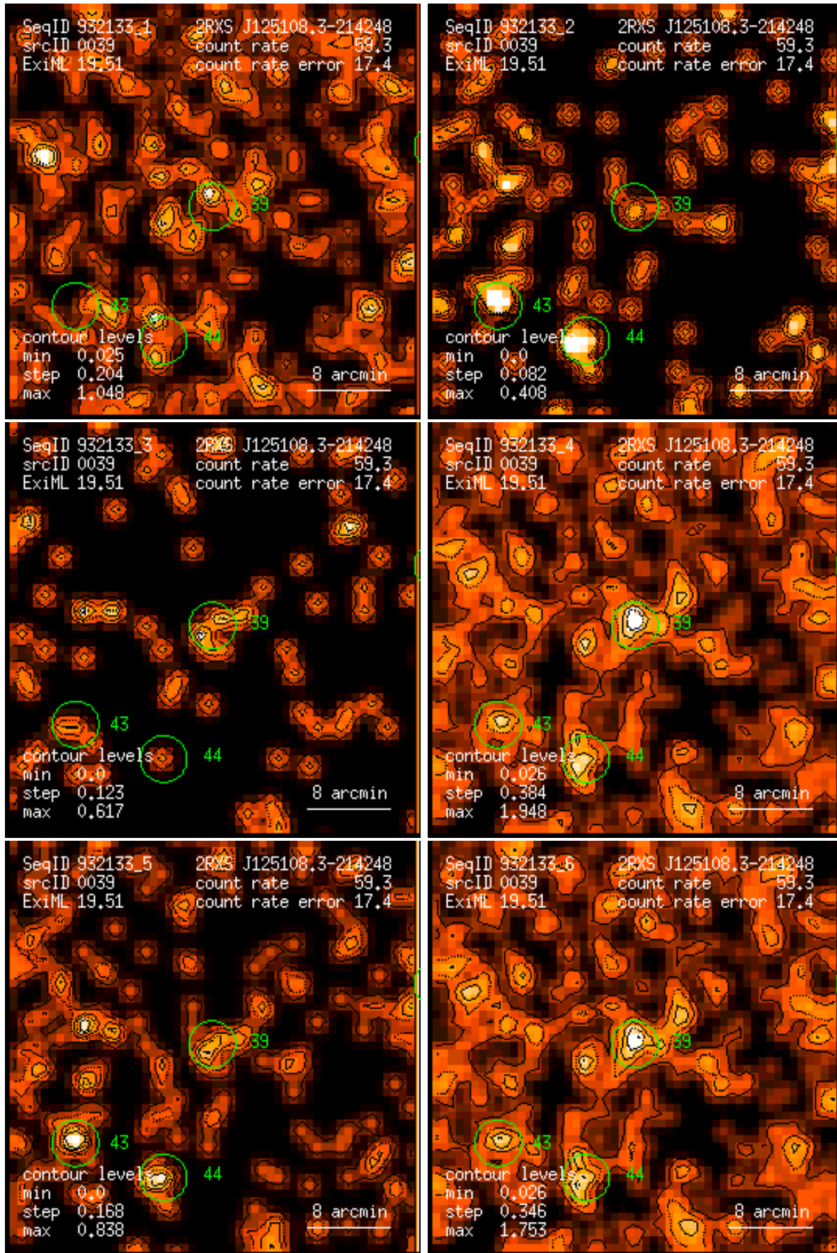
Figure 39: RASS 932133: detection 0039: band rate images, Gaussian filter: (1) PSPC channels 11 – 41, (2) 52 – 90, (3) 91 – 201, (4) 11 – 235, (5) 52 – 201, (6) 11 – 201. Broad band rates in counts/ks. Band rate contour levels in counts/ks/arcmin 2 .
