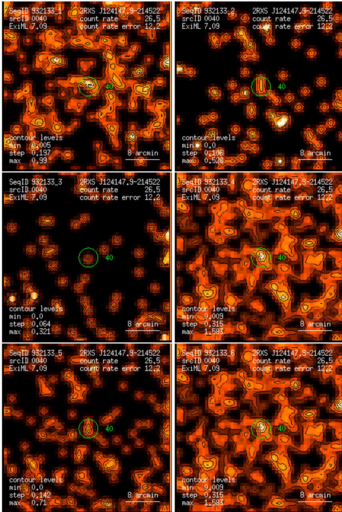
Figure 40: RASS 932133: detection 0040: band rate images, Gaussian filter: (1) PSPC channels 11 – 41, (2) 52 – 90, (3) 91 – 201, (4) 11 – 235, (5) 52 – 201, (6) 11 – 201. Broad band rates in counts/ks. Band rate contour levels in counts/ks/arcmin 2 .
