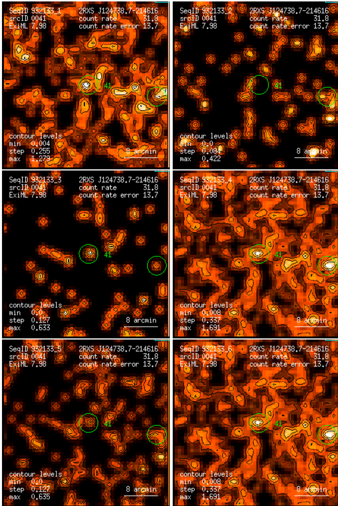
Figure 41: RASS 932133: detection 0041: band rate images, Gaussian filter: (1) PSPC channels 11 – 41, (2) 52 – 90, (3) 91 – 201, (4) 11 – 235, (5) 52 – 201, (6) 11 – 201. Broad band rates in counts/ks. Band rate contour levels in counts/ks/arcmin 2 .
