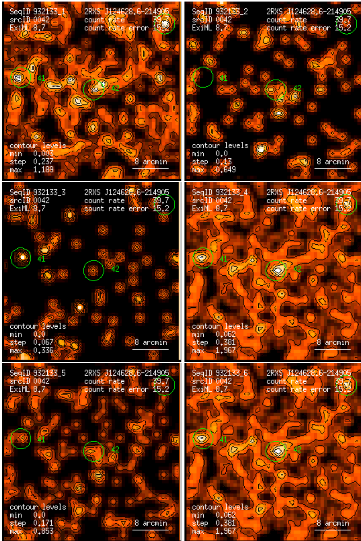
Figure 42: RASS 932133: detection 0042: band rate images, Gaussian filter: (1) PSPC channels 11 – 41, (2) 52 – 90, (3) 91 – 201, (4) 11 – 235, (5) 52 – 201, (6) 11 – 201. Broad band rates in counts/ks. Band rate contour levels in counts/ks/arcmin 2 .
