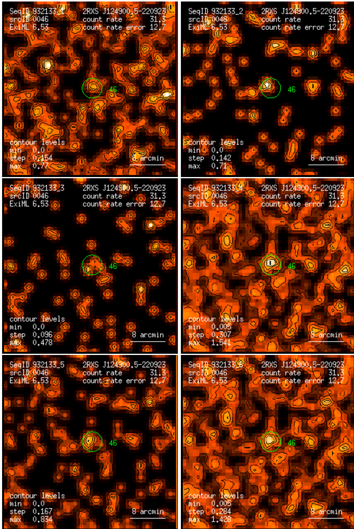
Figure 46: RASS 932133: detection 0046: band rate images, Gaussian filter: (1) PSPC channels 11 – 41, (2) 52 – 90, (3) 91 – 201, (4) 11 – 235, (5) 52 – 201, (6) 11 – 201. Broad band rates in counts/ks. Band rate contour levels in counts/ks/arcmin 2 .
