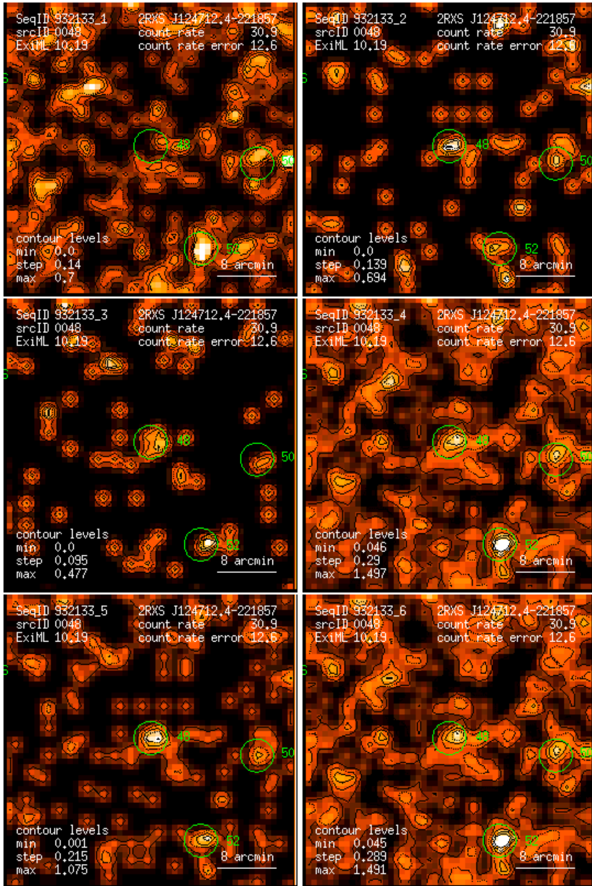
Figure 48: RASS 932133: detection 0048: band rate images, Gaussian filter: (1) PSPC channels 11 – 41, (2) 52 – 90, (3) 91 – 201, (4) 11 – 235, (5) 52 – 201, (6) 11 – 201. Broad band rates in counts/ks. Band rate contour levels in counts/ks/arcmin 2 .
