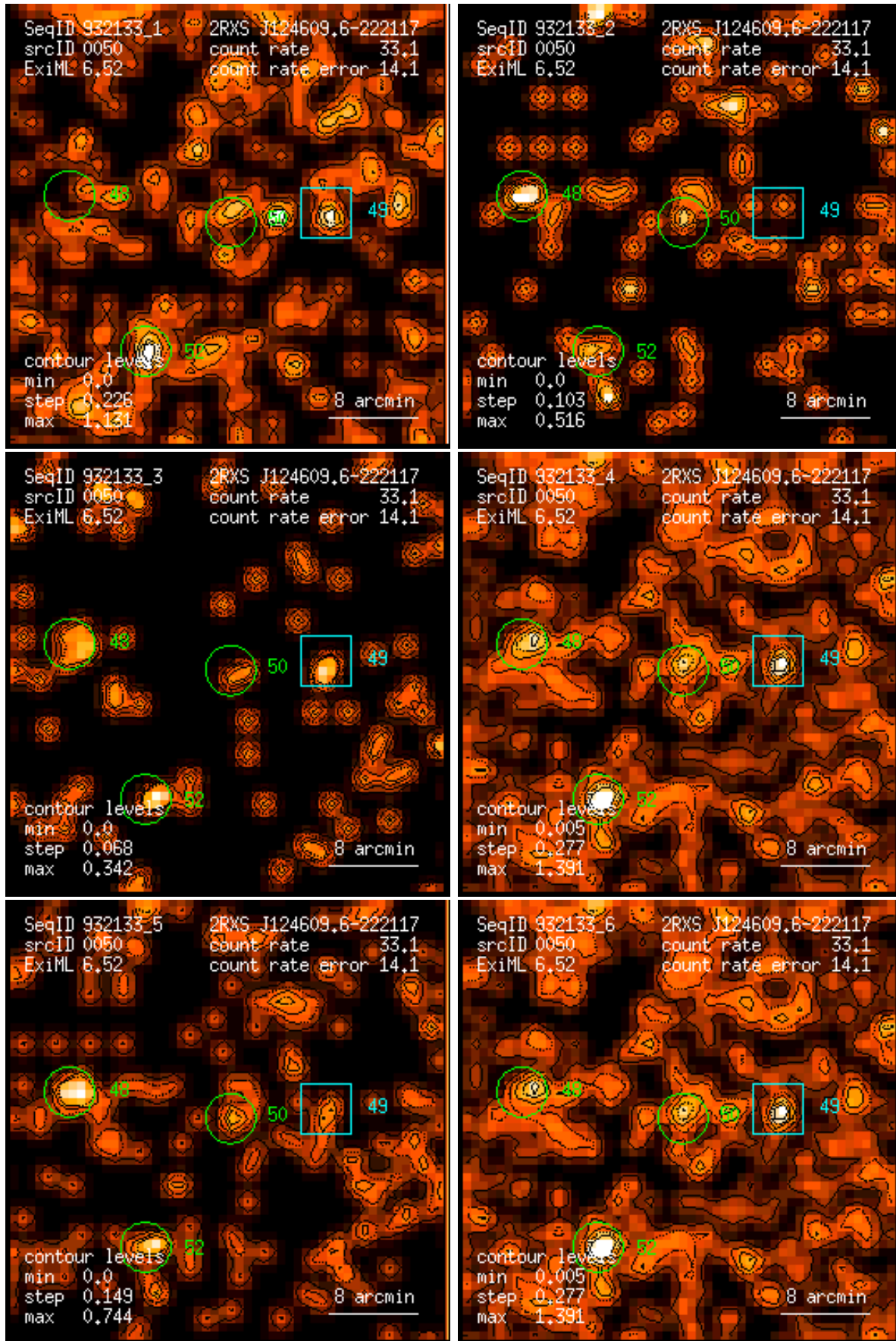
Figure 50: RASS 932133: detection 0050: band rate images, Gaussian filter: (1) PSPC channels 11 – 41, (2) 52 – 90, (3) 91 – 201, (4) 11 – 235, (5) 52 – 201, (6) 11 – 201. Broad band rates in counts/ks. Band rate contour levels in counts/ks/arcmin 2 .
