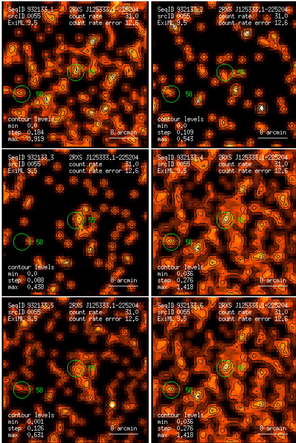
Figure 55: RASS 932133: detection 0055: band rate images, Gaussian filter: (1) PSPC channels 11 – 41, (2) 52 – 90, (3) 91 – 201, (4) 11 – 235, (5) 52 – 201, (6) 11 – 201. Broad band rates in counts/ks. Band rate contour levels in counts/ks/arcmin 2 .
