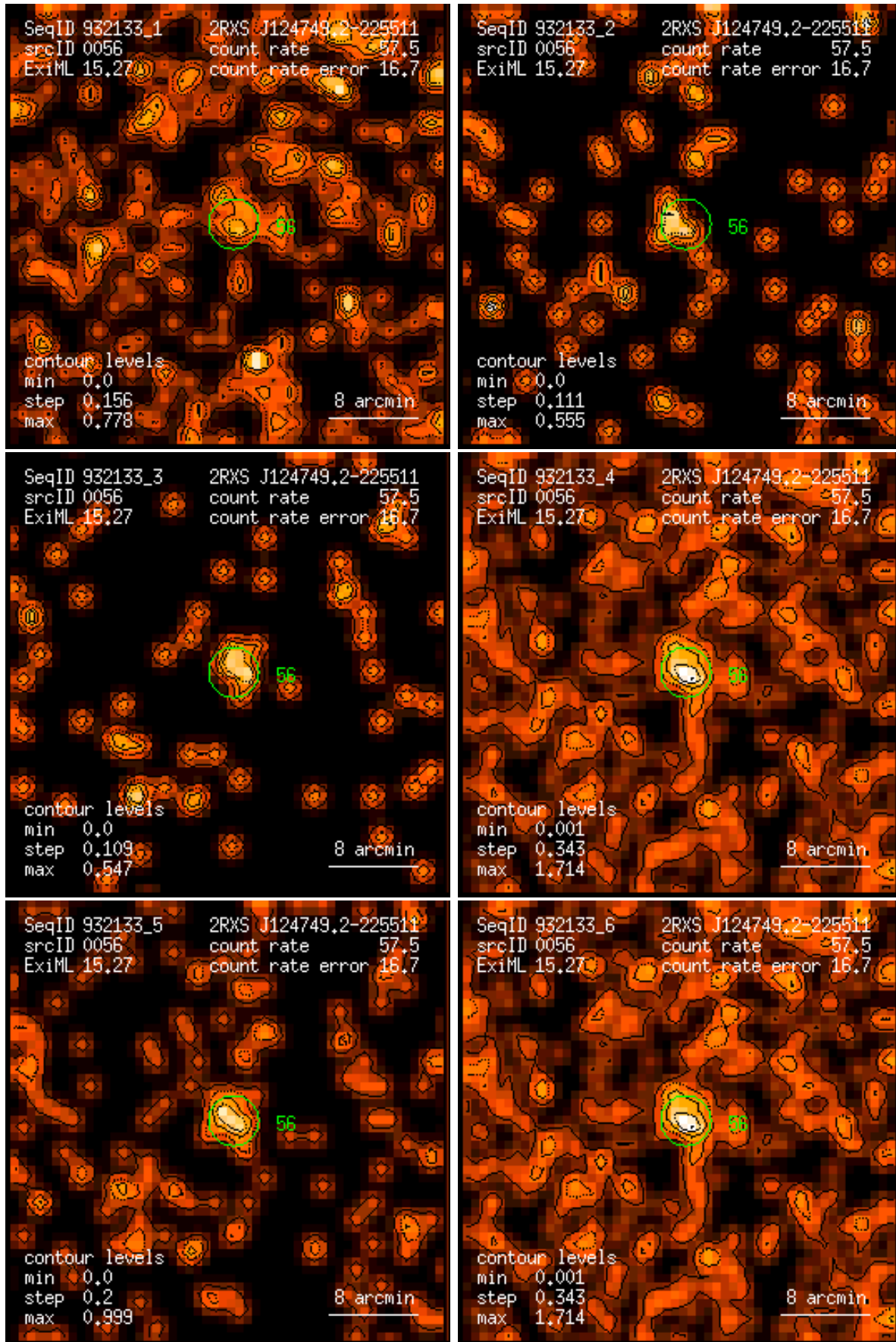
Figure 56: RASS 932133: detection 0056: band rate images, Gaussian filter: (1) PSPC channels 11 – 41, (2) 52 – 90, (3) 91 – 201, (4) 11 – 235, (5) 52 – 201, (6) 11 – 201. Broad band rates in counts/ks. Band rate contour levels in counts/ks/arcmin 2 .
