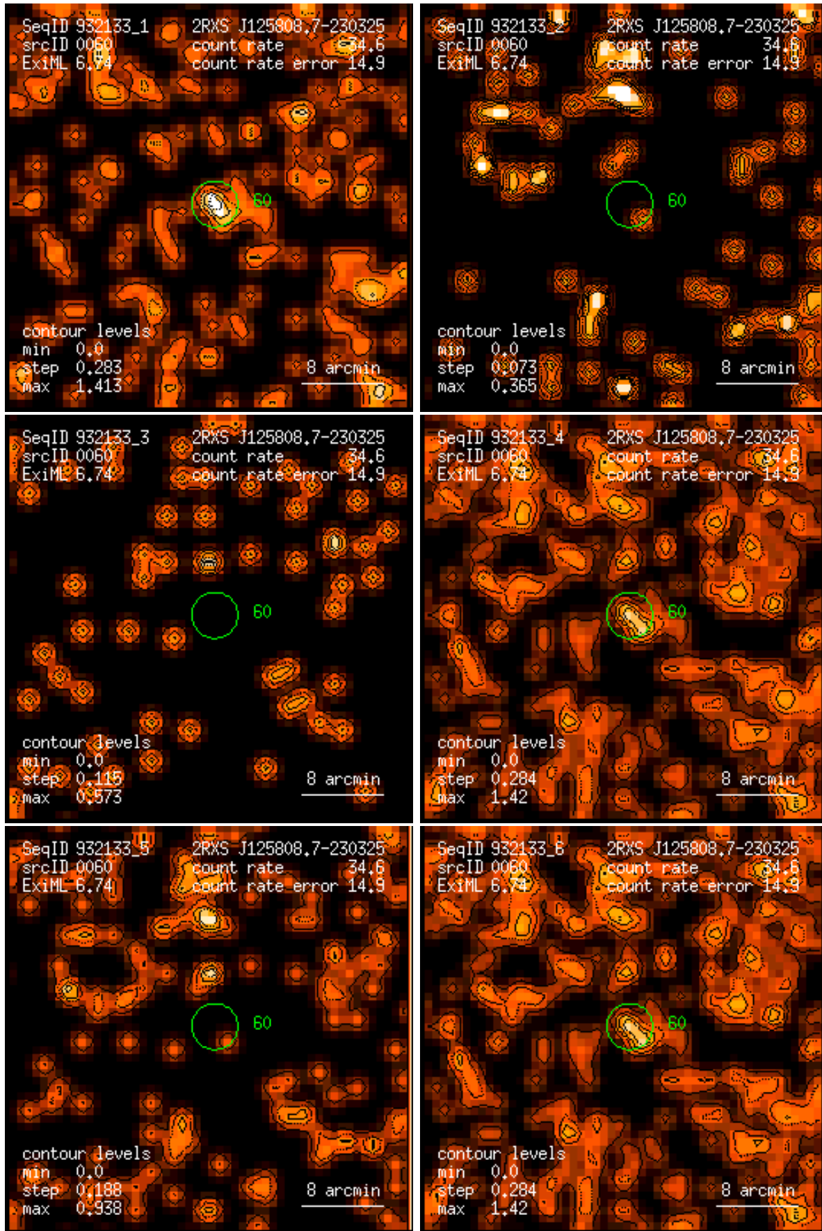
Figure 60: RASS 932133: detection 0060: band rate images, Gaussian filter: (1) PSPC channels 11 – 41, (2) 52 – 90, (3) 91 – 201, (4) 11 – 235, (5) 52 – 201, (6) 11 – 201. Broad band rates in counts/ks. Band rate contour levels in counts/ks/arcmin 2 .
