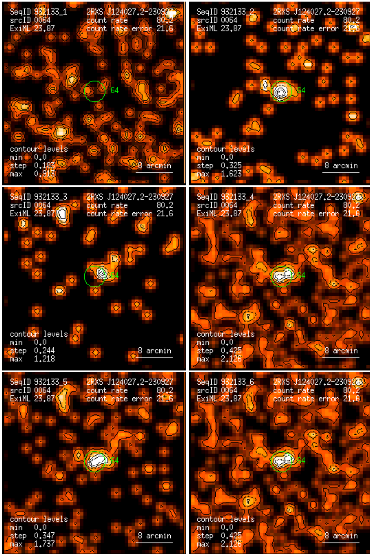
Figure 64: RASS 932133: detection 0064: band rate images, Gaussian filter: (1) PSPC channels 11 – 41, (2) 52 – 90, (3) 91 – 201, (4) 11 – 235, (5) 52 – 201, (6) 11 – 201. Broad band rates in counts/ks. Band rate contour levels in counts/ks/arcmin 2 .
