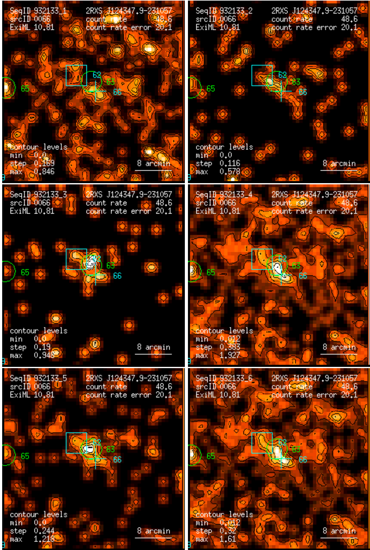
Figure 66: RASS 932133: detection 0066: band rate images, Gaussian filter: (1) PSPC channels 11 – 41, (2) 52 – 90, (3) 91 – 201, (4) 11 – 235, (5) 52 – 201, (6) 11 – 201. Broad band rates in counts/ks. Band rate contour levels in counts/ks/arcmin 2 .
