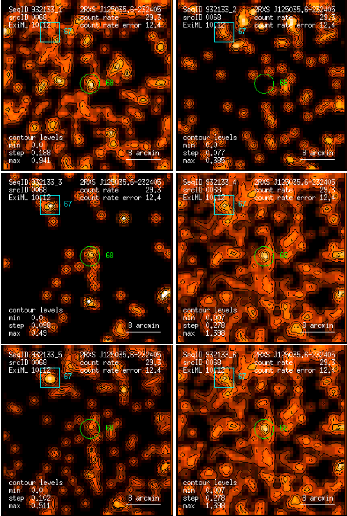
Figure 68: RASS 932133: detection 0068: band rate images, Gaussian filter: (1) PSPC channels 11 – 41, (2) 52 – 90, (3) 91 – 201, (4) 11 – 235, (5) 52 – 201, (6) 11 – 201. Broad band rates in counts/ks. Band rate contour levels in counts/ks/arcmin 2 .
