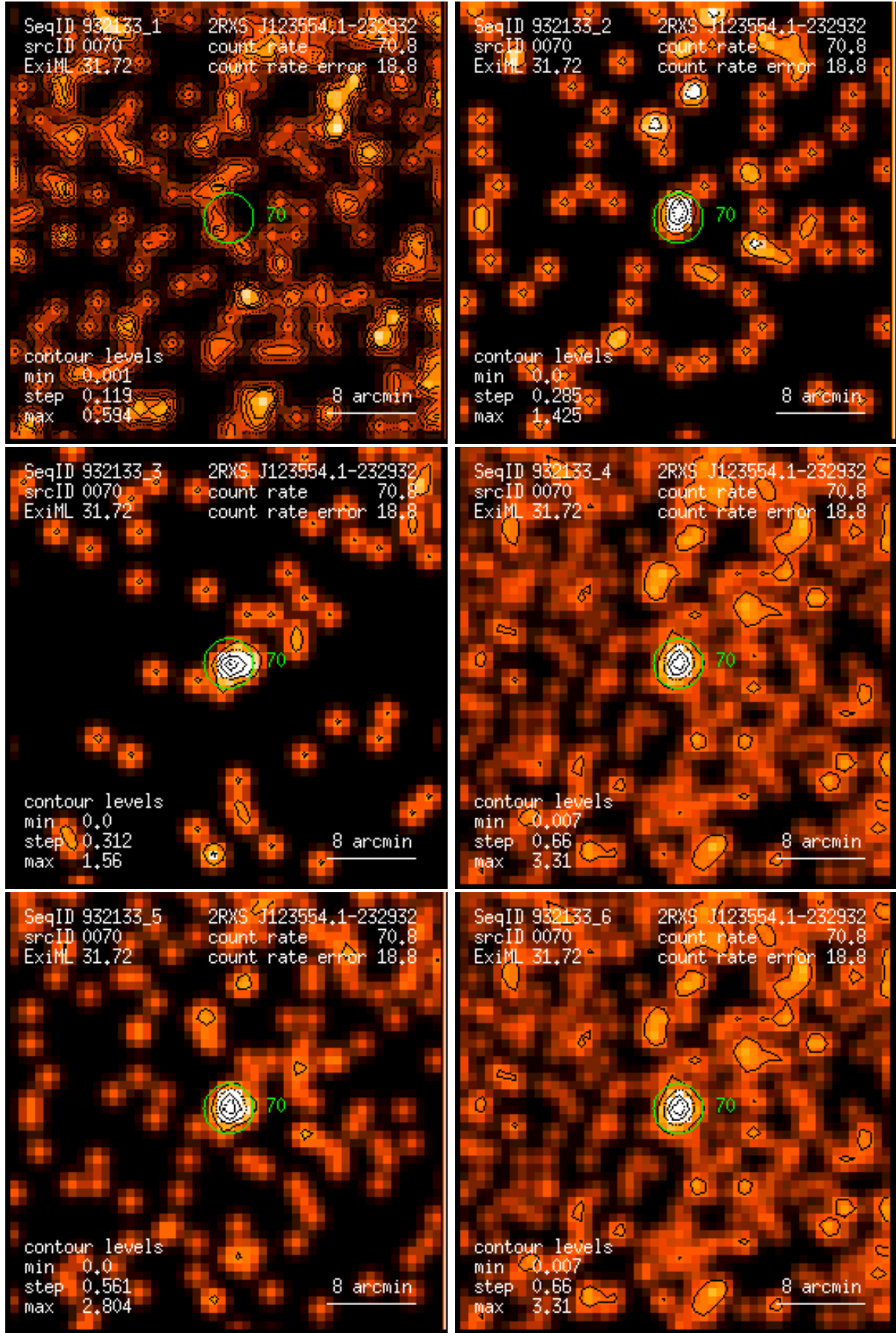
Figure 70: RASS 932133: detection 0070: band rate images, Gaussian filter: (1) PSPC channels 11 – 41, (2) 52 – 90, (3) 91 – 201, (4) 11 – 235, (5) 52 – 201, (6) 11 – 201. Broad band rates in counts/ks. Band rate contour levels in counts/ks/arcmin 2 .
