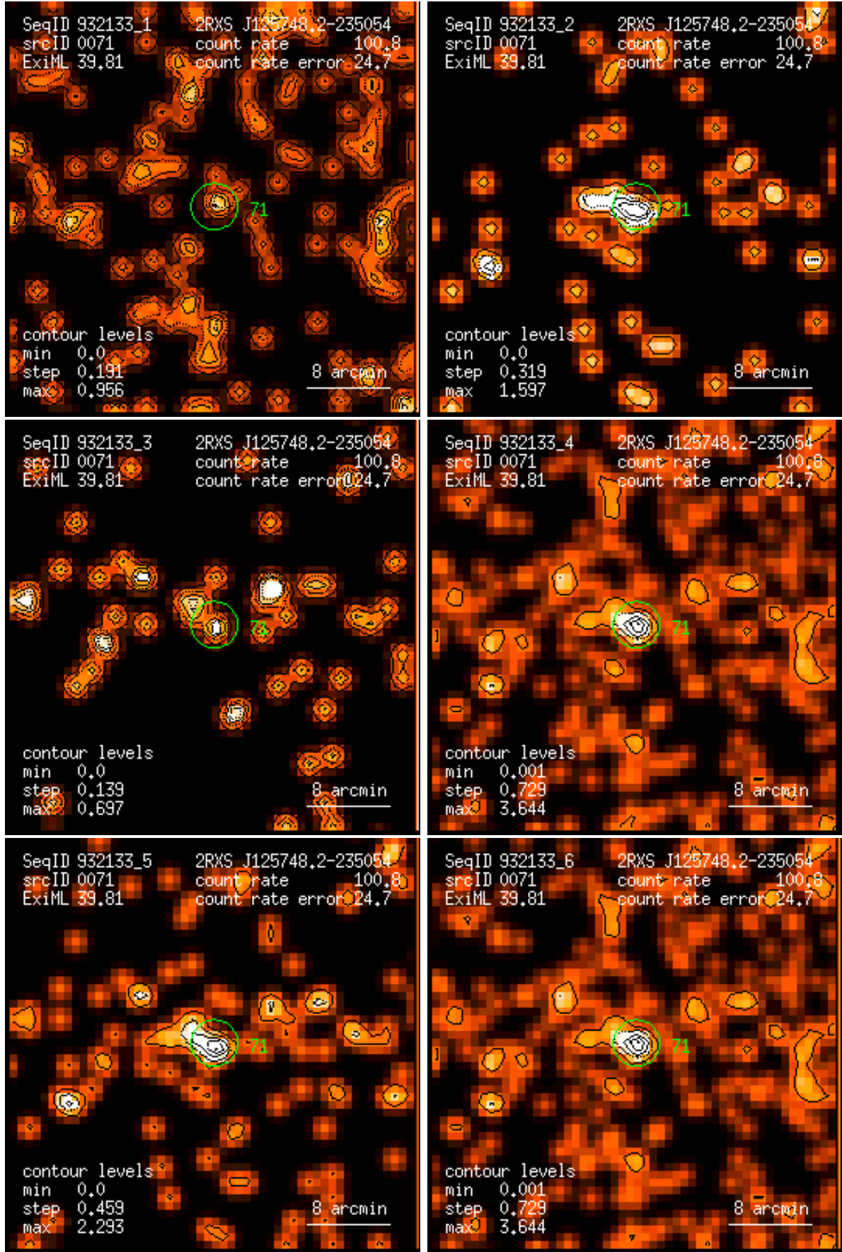
Figure 71: RASS 932133: detection 0071: band rate images, Gaussian filter: (1) PSPC channels 11 – 41, (2) 52 – 90, (3) 91 – 201, (4) 11 – 235, (5) 52 – 201, (6) 11 – 201. Broad band rates in counts/ks. Band rate contour levels in counts/ks/arcmin 2 .
