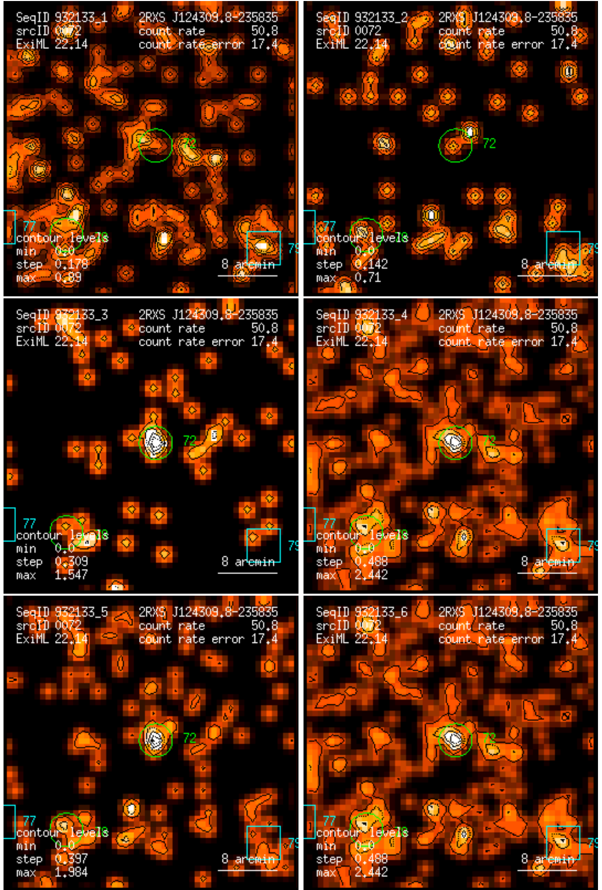
Figure 72: RASS 932133: detection 0072: band rate images, Gaussian filter: (1) PSPC channels 11 – 41, (2) 52 – 90, (3) 91 – 201, (4) 11 – 235, (5) 52 – 201, (6) 11 – 201. Broad band rates in counts/ks. Band rate contour levels in counts/ks/arcmin 2 .
