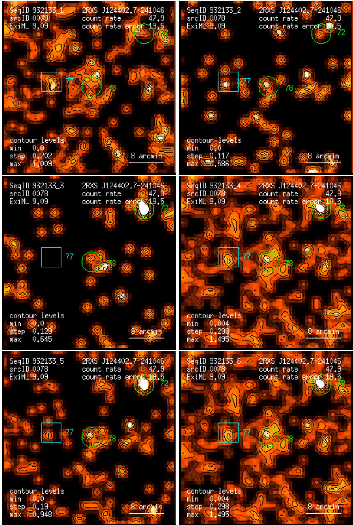
Figure 78: RASS 932133: detection 0078: band rate images, Gaussian filter: (1) PSPC channels 11 – 41, (2) 52 – 90, (3) 91 – 201, (4) 11 – 235, (5) 52 – 201, (6) 11 – 201. Broad band rates in counts/ks. Band rate contour levels in counts/ks/arcmin 2 .
