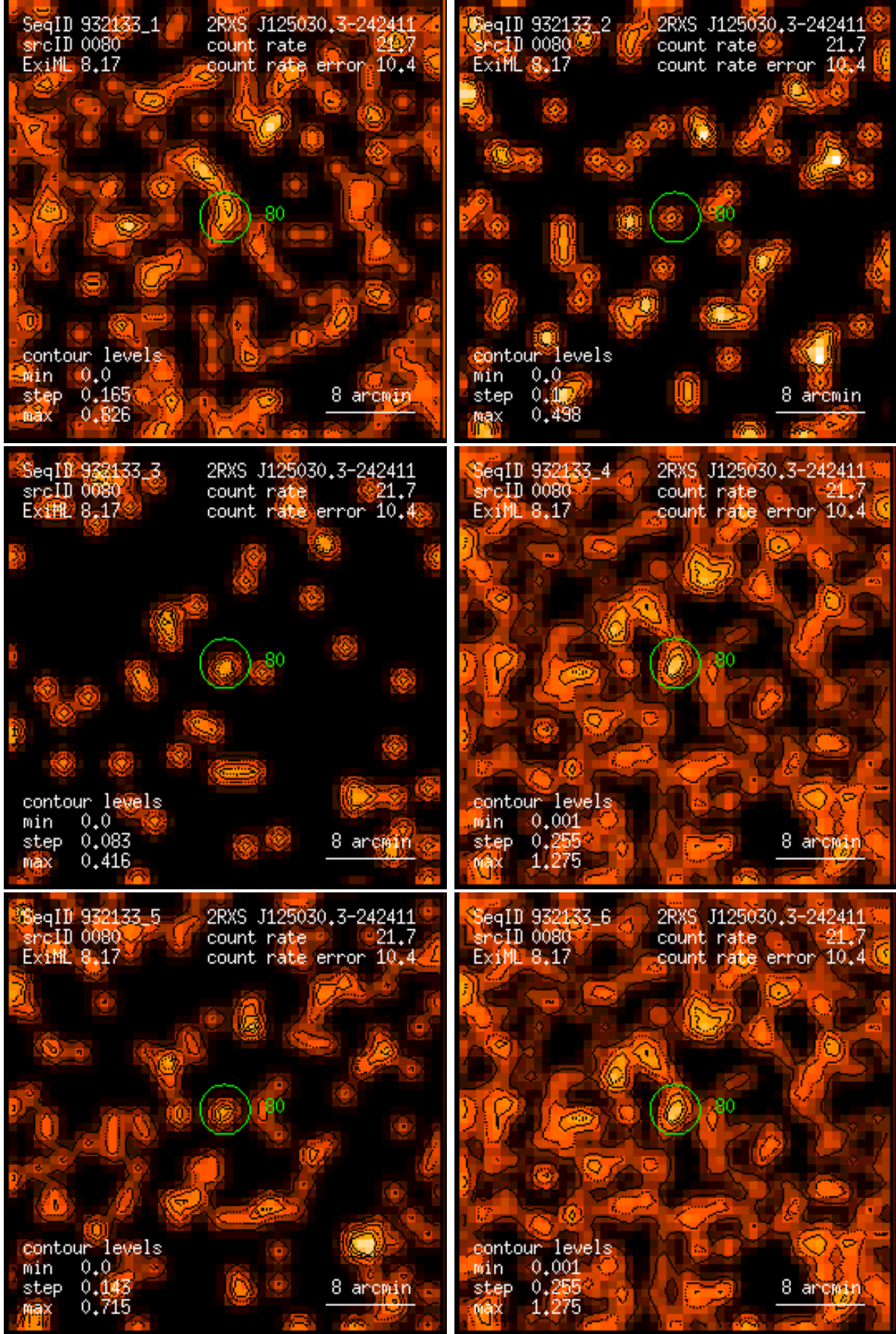
Figure 80: RASS 932133: detection 0080: band rate images, Gaussian filter: (1) PSPC channels 11 – 41, (2) 52 – 90, (3) 91 – 201, (4) 11 – 235, (5) 52 – 201, (6) 11 – 201. Broad band rates in counts/ks. Band rate contour levels in counts/ks/arcmin 2 .
