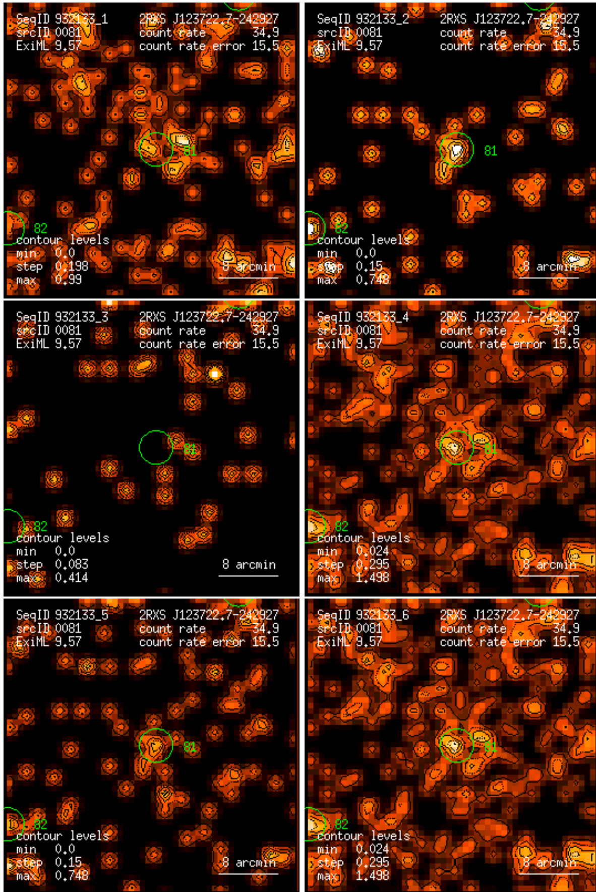
Figure 81: RASS 932133: detection 0081: band rate images, Gaussian filter: (1) PSPC channels 11 – 41, (2) 52 – 90, (3) 91 – 201, (4) 11 – 235, (5) 52 – 201, (6) 11 – 201. Broad band rates in counts/ks. Band rate contour levels in counts/ks/arcmin 2 .
